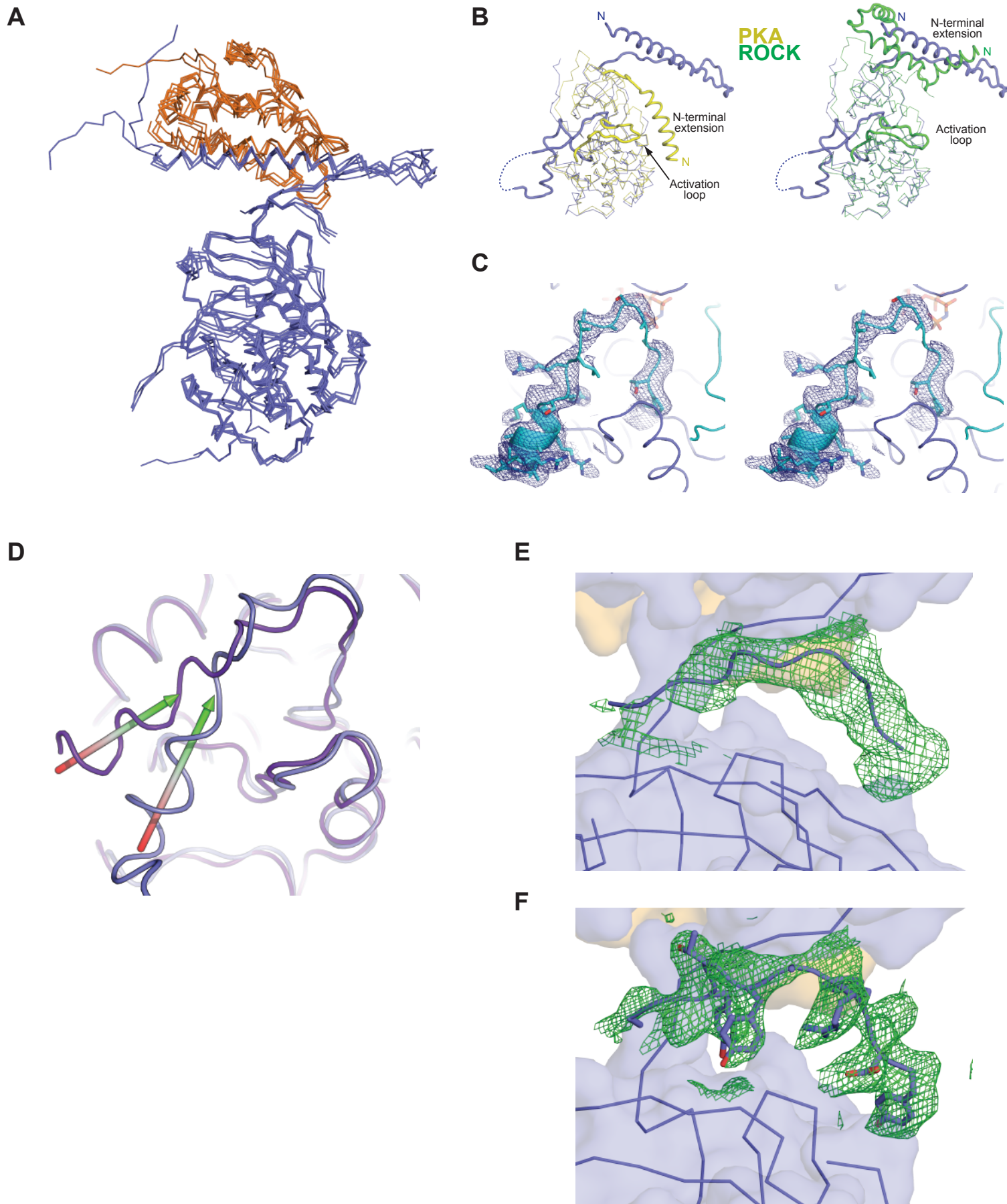
Figure S2. Additional information on the crystal structures of Cbk1–Mob2 complexes
