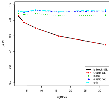
Figure S1 The mean pAUC versus the size of the LD block containing a single causal SNP sigBlock for the proposed method (“ld block-GL”, black solid lines), oracle Group Lasso (dashed red lines), Lasso (dotted green lines), Elastic-Net (dash-dotted blue lines) and SMA (“univ”, dashed light blue lines), for \rho = 0.4 . Left: SNP-level evaluation. Right: block-level evaluation.
