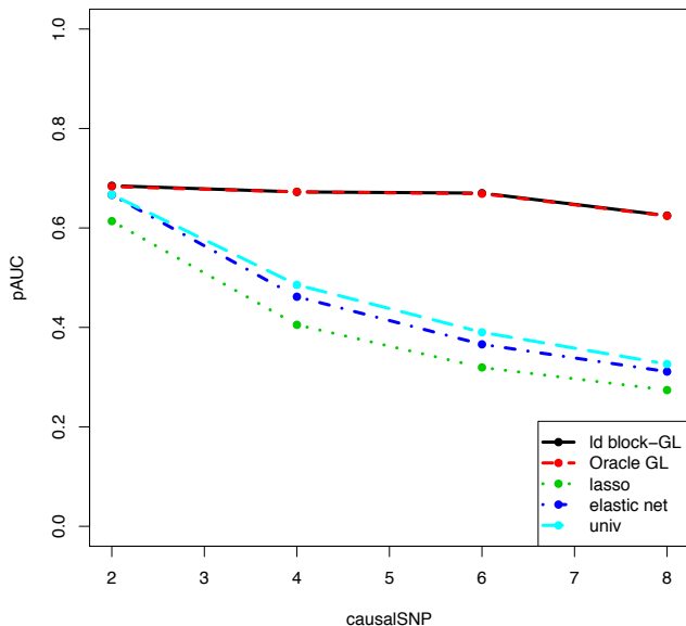
Figure S2 The mean pAUC as a function of the number of causal SNPs causalSNP within a block of size 8, for the proposed method (“ld block-GL”, black solid lines), oracle Group Lasso (dashed red lines), Lasso (dotted green lines), Elastic-Net (dash-dotted blue lines) and SMA (“univ”, dashed light blue lines), for \rho = 0.4 .
