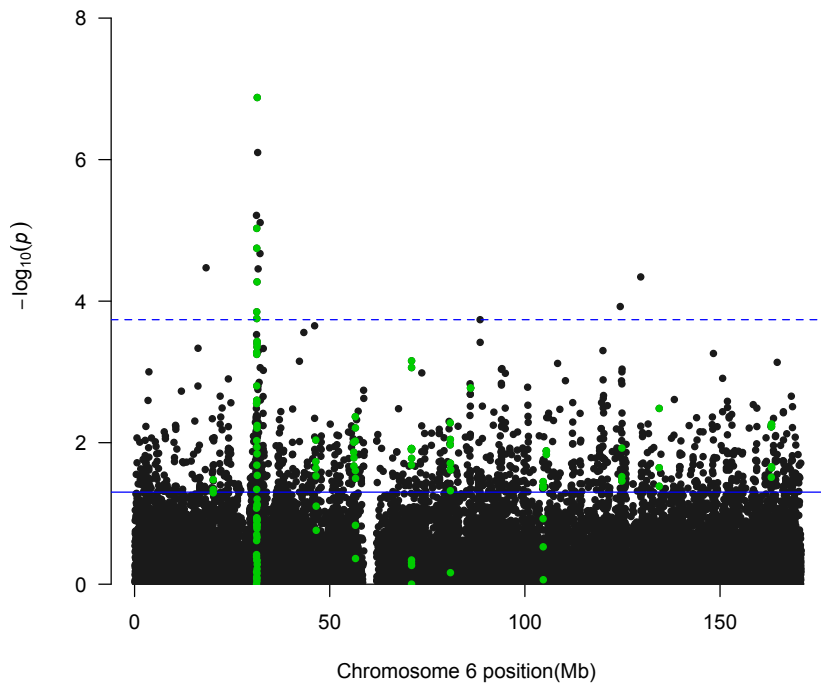
Figure S3 Manhattan plot for the HIV data results. The markers highlighted in green correspond to the SNPs of the first 15 blocks selected by the proposed approach on the MHC region.
