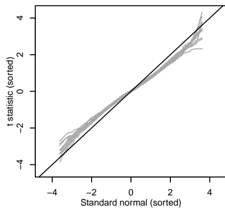
C. t(\text{Time0}) in P. stutzeri
