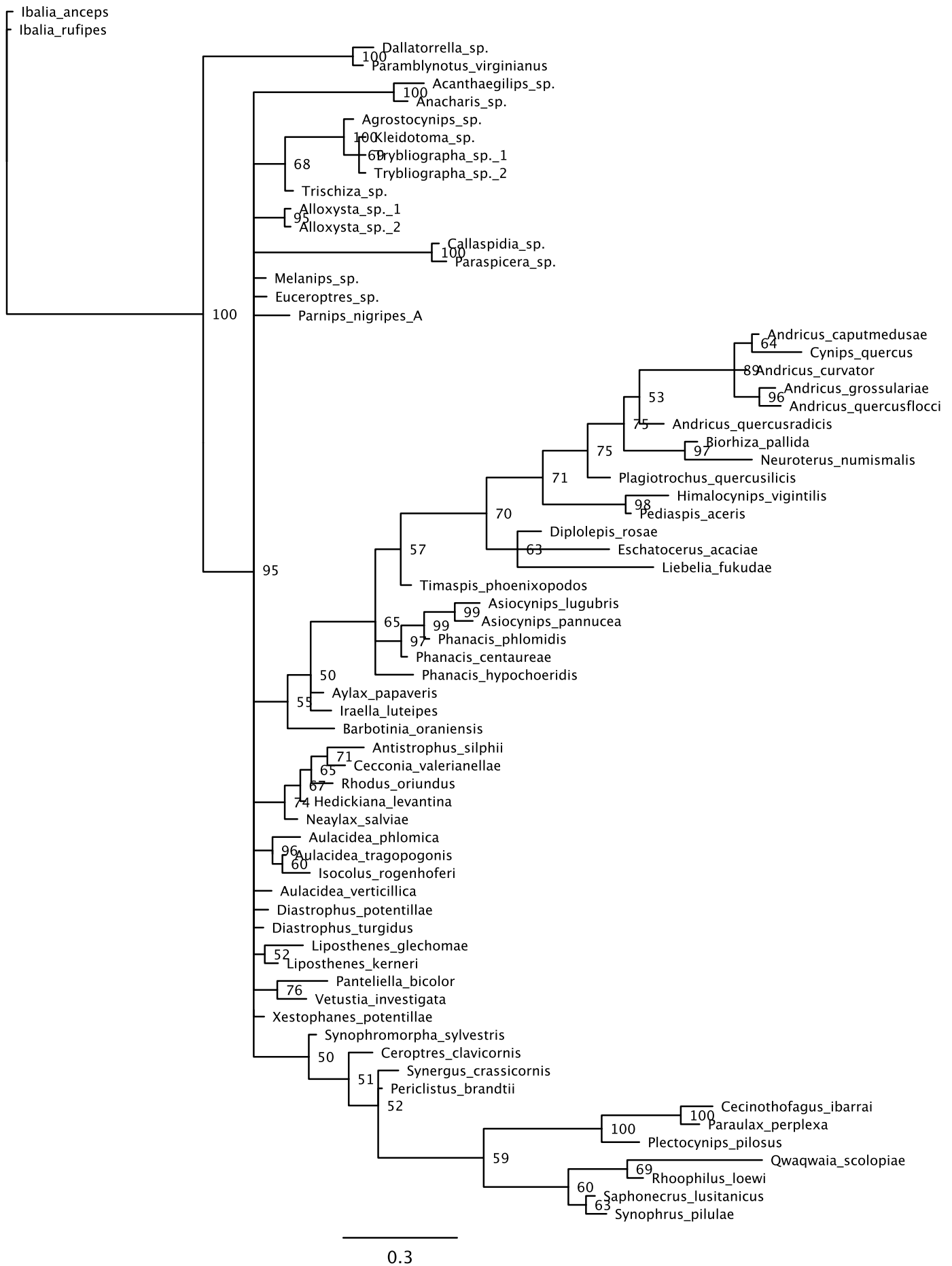
S6 Figure. Tree based on morphology, without biological data, with posterior clade probabilities (%) on branches.
