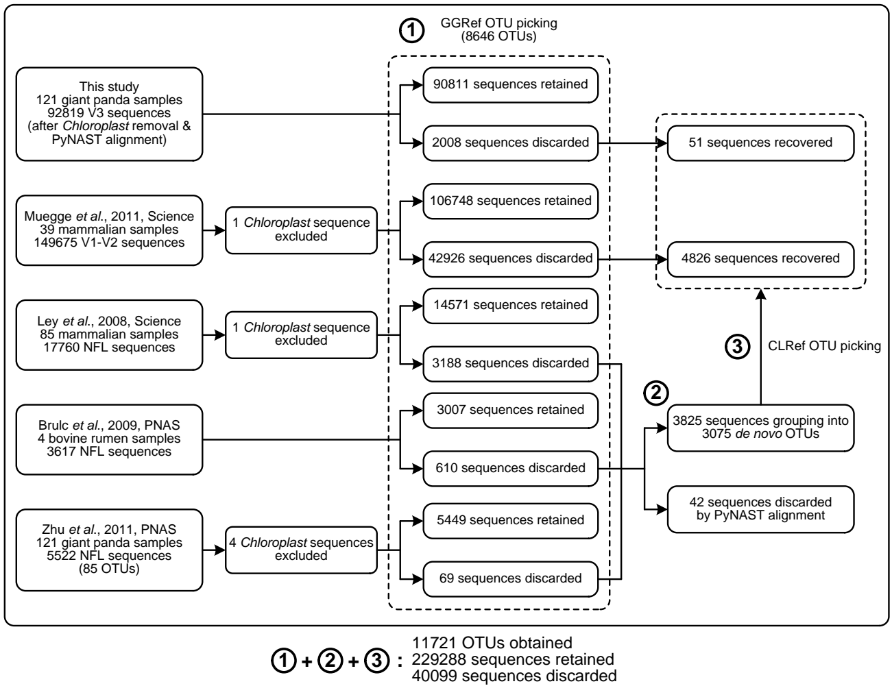
Figure S4 The pipeline of the multi-step OTU picking procedure. GGRef denotes the reference-based OTU picking against the Greengenes reference database, whereas CLRef denotes the reference-based OTU picking against the 3,075 OTUs derived from the GGRef-discarded sequences from the three clone library datasets. NFL, near full-length.
