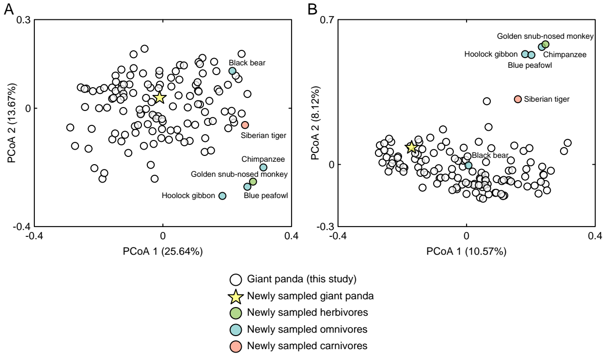
Figure S7 Comparison of gut microbiota structure of the giant panda population described in this study with that of the newly sampled herbivores, omnivores, and carnivores. PCoA score plots based on the weighted (A) and unweighted (B) UniFrac distances are shown.
