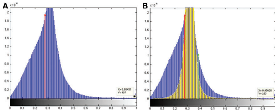
SUPPLEMENTARY FIG. S2. Pixel histograms for (A) representative images of cells containing LDs, shown in blue , and (B) overlaid with a histogram for a representative image of cells with no LDs, shown in yellow . It can be seen in the overlaid image that the blue histogram includes a shoulder to the right of the average, indicating that images with differentiated cells contain a larger fraction of bright pixels (due to the interior of LDs). The red line indicates the automatically determined threshold, and the green line indicates the high threshold set at a 15% higher value.
