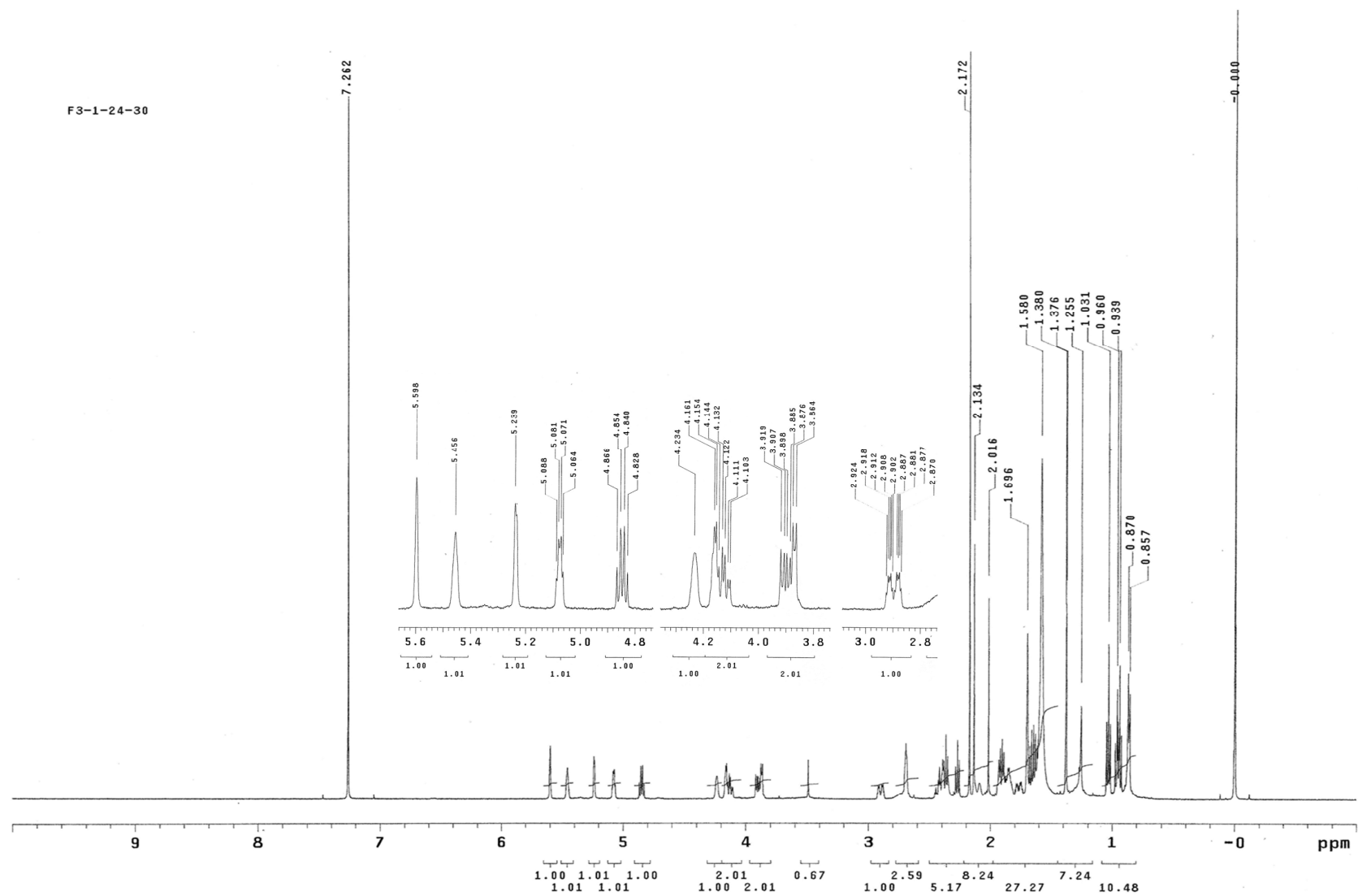
Figure S5. 1 H NMR spectrum of 2 in CDCl 3 .
