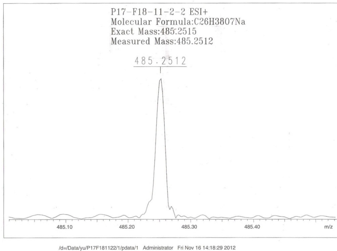
Figure S1. HRESIMS spectrum of 1 .
