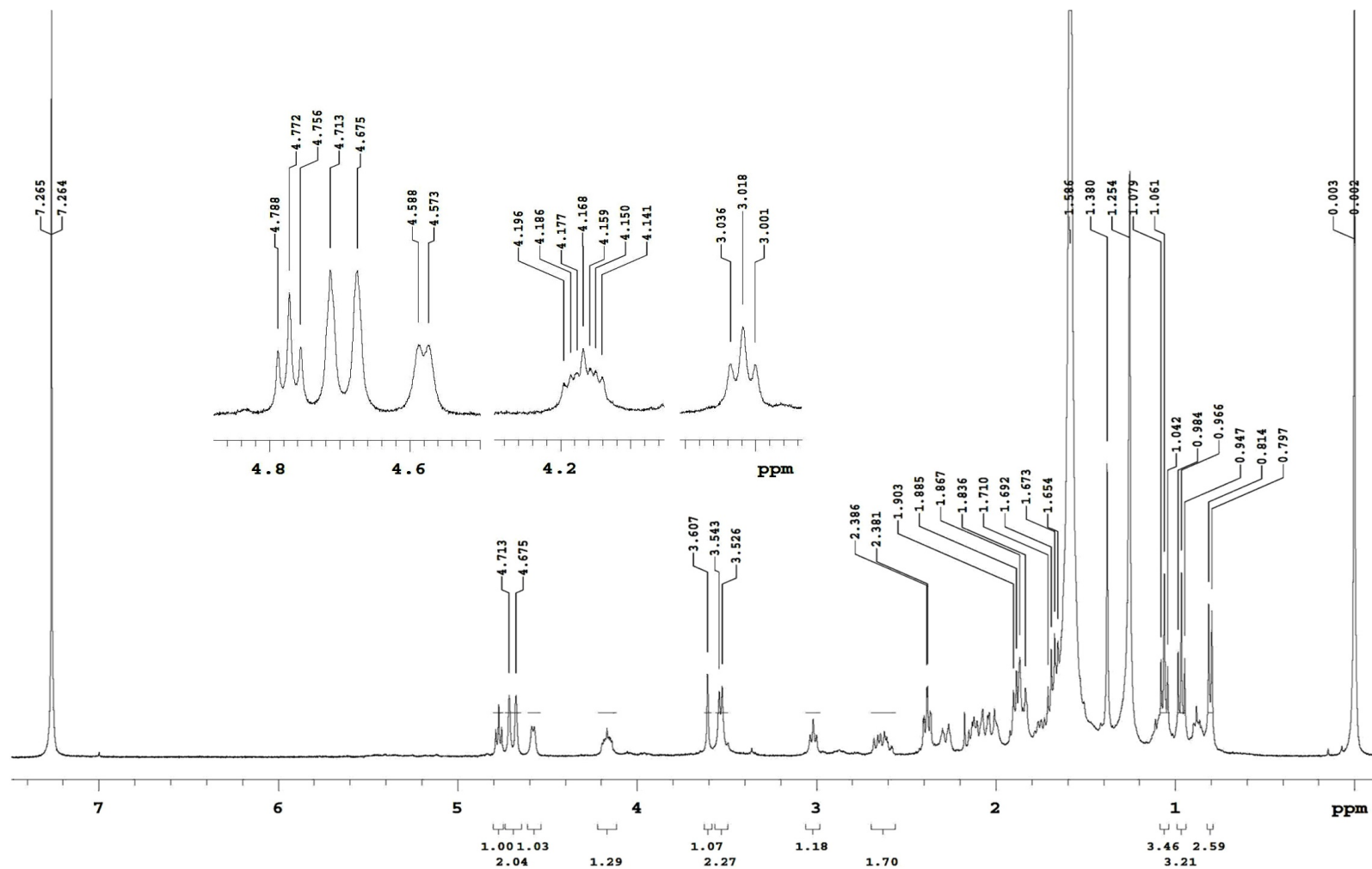
Figure S11. ^1\text{H} NMR spectrum of 4 in \text{CDCl}_3 .
