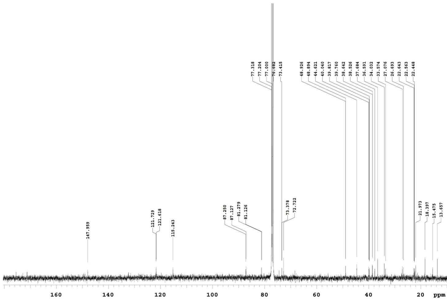
Figure S9. 13 C NMR spectrum of 3 in CDCl 3 .
