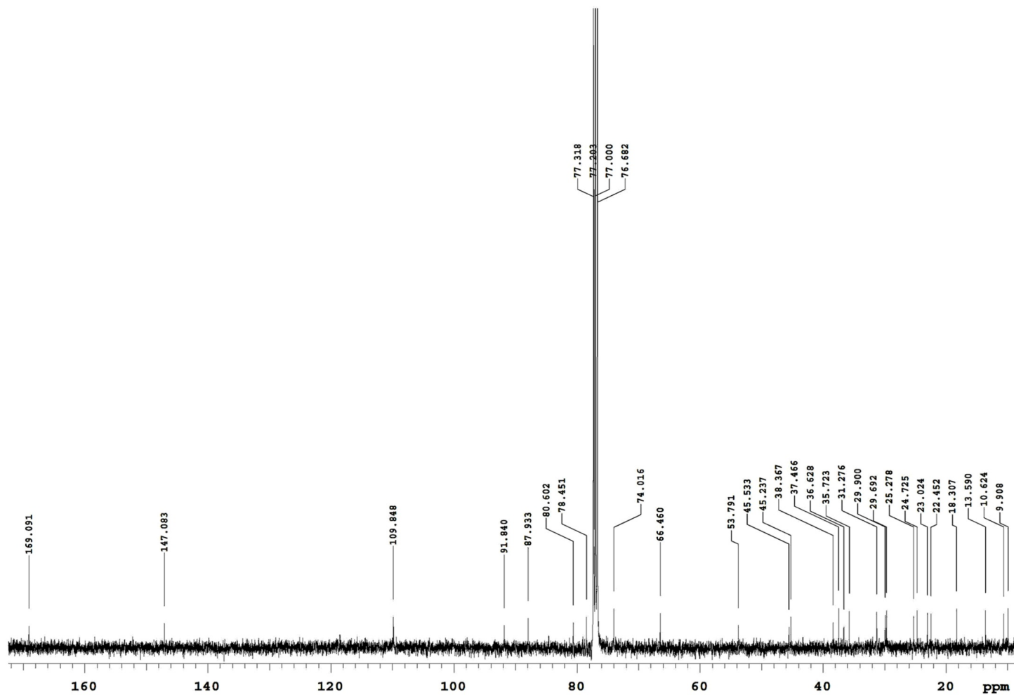
Figure S12. ^{13}\text{C} NMR spectrum of 4 in \text{CDCl}_3 .
