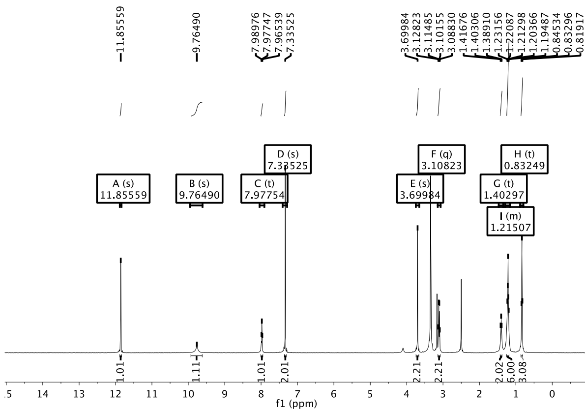
Figure S6. ^1\text{H-NMR} spectrum of N -hexyl-3-(3,5-dibromo-4-hydroxyphenyl)-2-(2-hydroxyimino)-propanamide ( 9 ).
