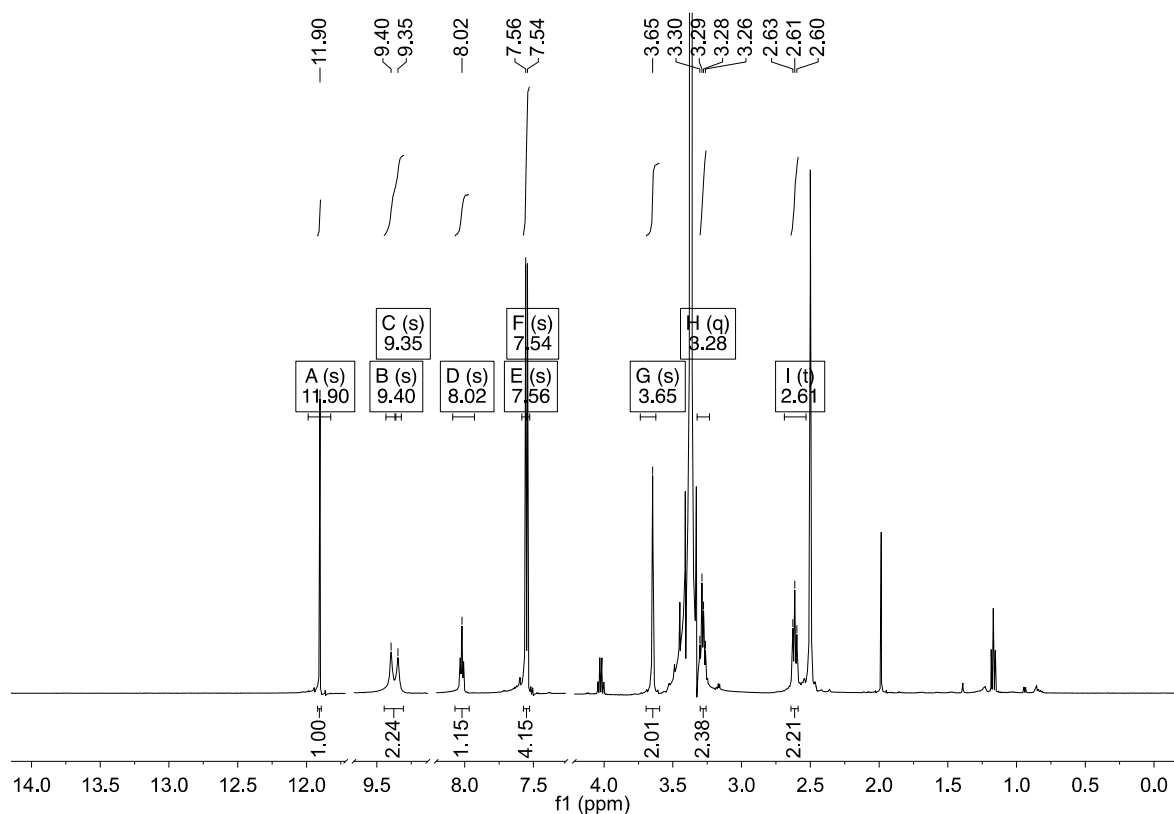
Figure S1. ^1\text{H-NMR} spectrum of tetraiodo-norbromohemibastadin-1 ( 4 ).
