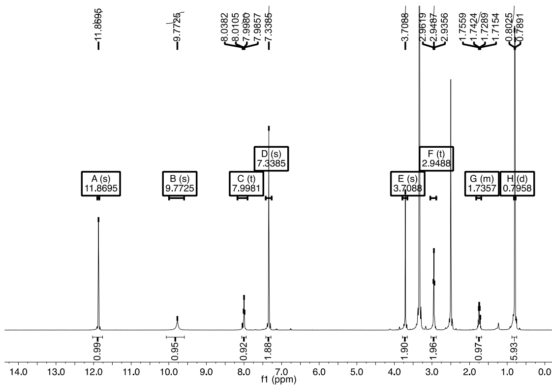
Figure S5. ^1\text{H-NMR} spectrum of N -(2-methyl-propyl)-3-(3,5-dibromo-4-hydroxyphenyl)-2-(2-hydroxyimino)-propanamide ( 8 ).
