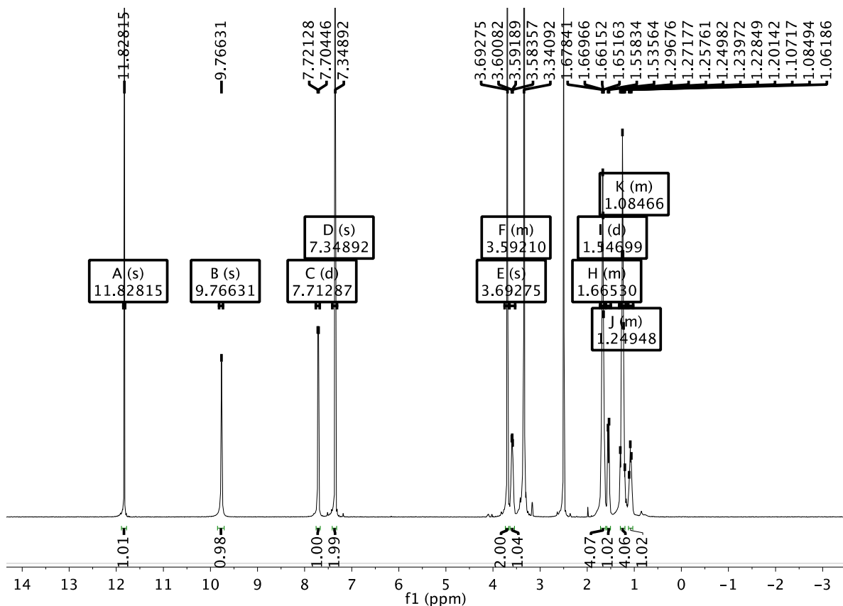
Figure S4. ^1\text{H-NMR} spectrum of N -cyclohexyl-3-(3,5-dibromo-4-hydroxyphenyl)-2-(2-hydroxyimino)-propanamide ( 7 ).
