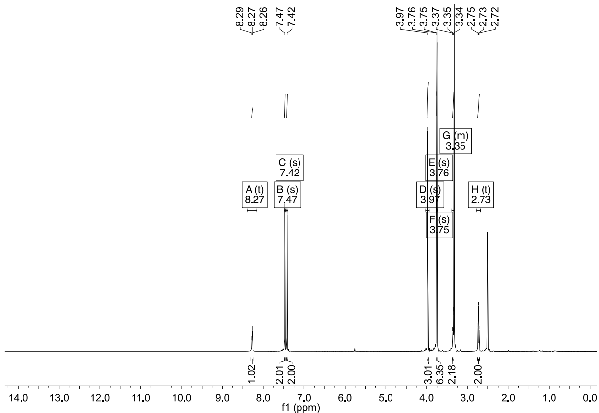
Figure S3. ^1\text{H-NMR} spectrum of trimethoxy-5,5'-dibromohemibastadin-1 ( 6 ).
