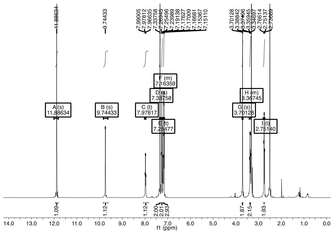
Figure S7. ^1\text{H-NMR} spectrum of N -2-phenylethyl-3-(3,5-dibromo-4-hydroxyphenyl)-2-(2-hydroxyimino)-propanamide ( 10 ).
