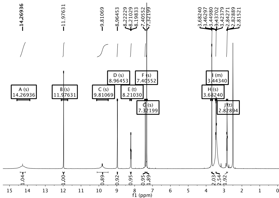
Figure S8. ^1\text{H-NMR} spectrum of N -[2-(4-imidazolyl)-ethyl]-3-(3,5-dibromo-4-hydroxyphenyl)-2-(2-hydroxyimino)-propanamide ( 11 ).
