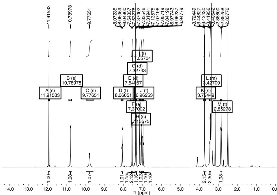
Figure S9. ^1\text{H-NMR} spectrum of N -[2-(3-indolyl)-ethyl]-3-(3,5-dibromo-4-hydroxyphenyl)-2-(2-hydroxyimino)-propanamide ( 12 ).
