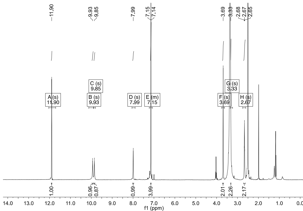
Figure S2. ^1\text{H-NMR} spectrum of tetrachloro-norbromohemibastadin-1 ( 5 ).
