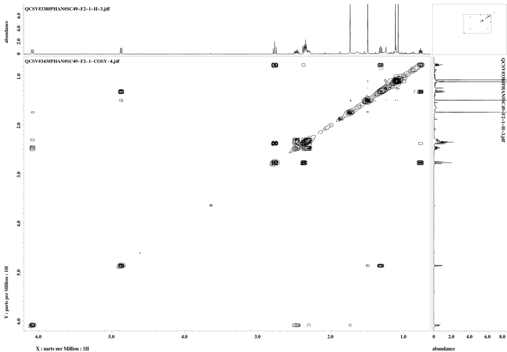
Figure S5. ^1\text{H} - ^1\text{H} COSY spectrum of capgermacrene A ( 1 ) in \text{CDCl}_3 .
