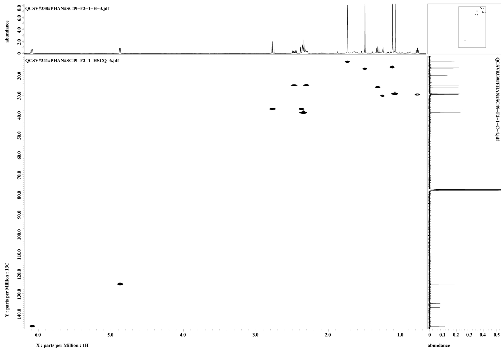
Figure S4. HSQC spectrum of capgermacrene A (1) in \text{CDCl}_3 .
