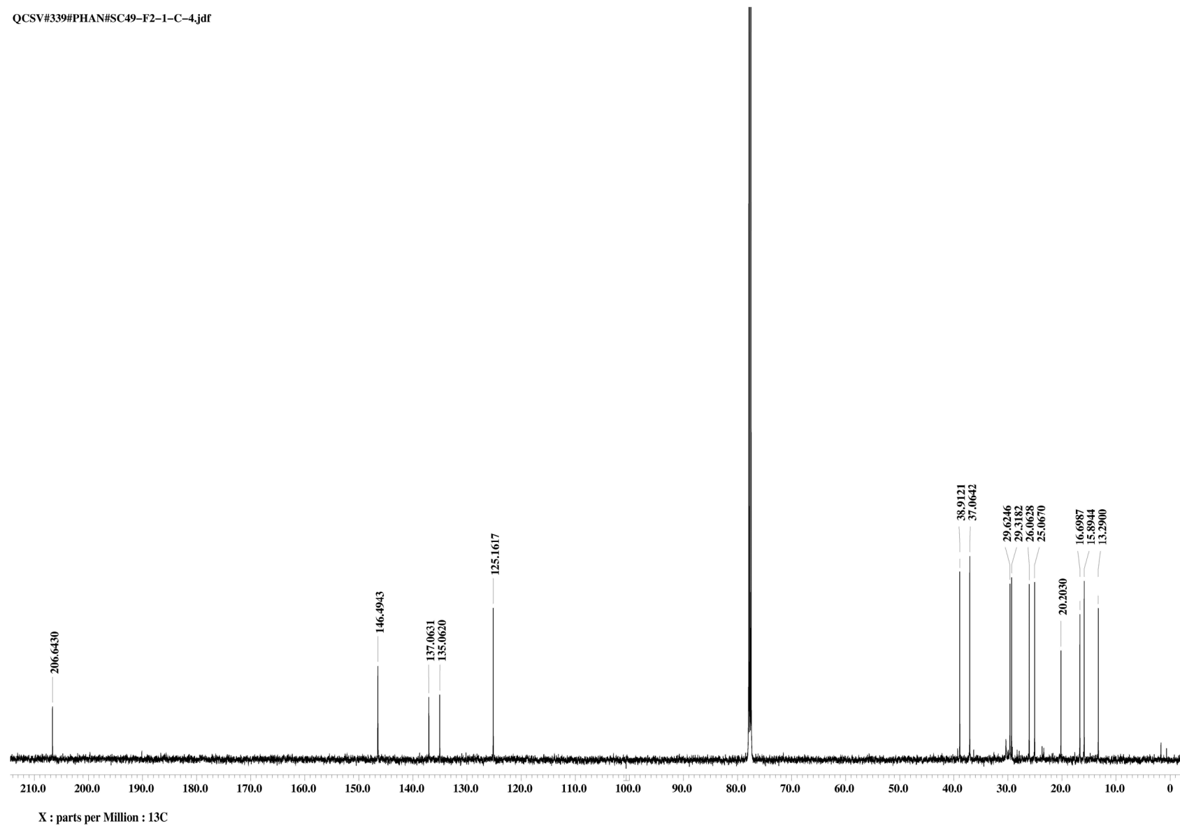
Figure S2. ^{13}\text{C} -NMR spectrum of capgermacrene A (1) in \text{CDCl}_3 (150 MHz).
