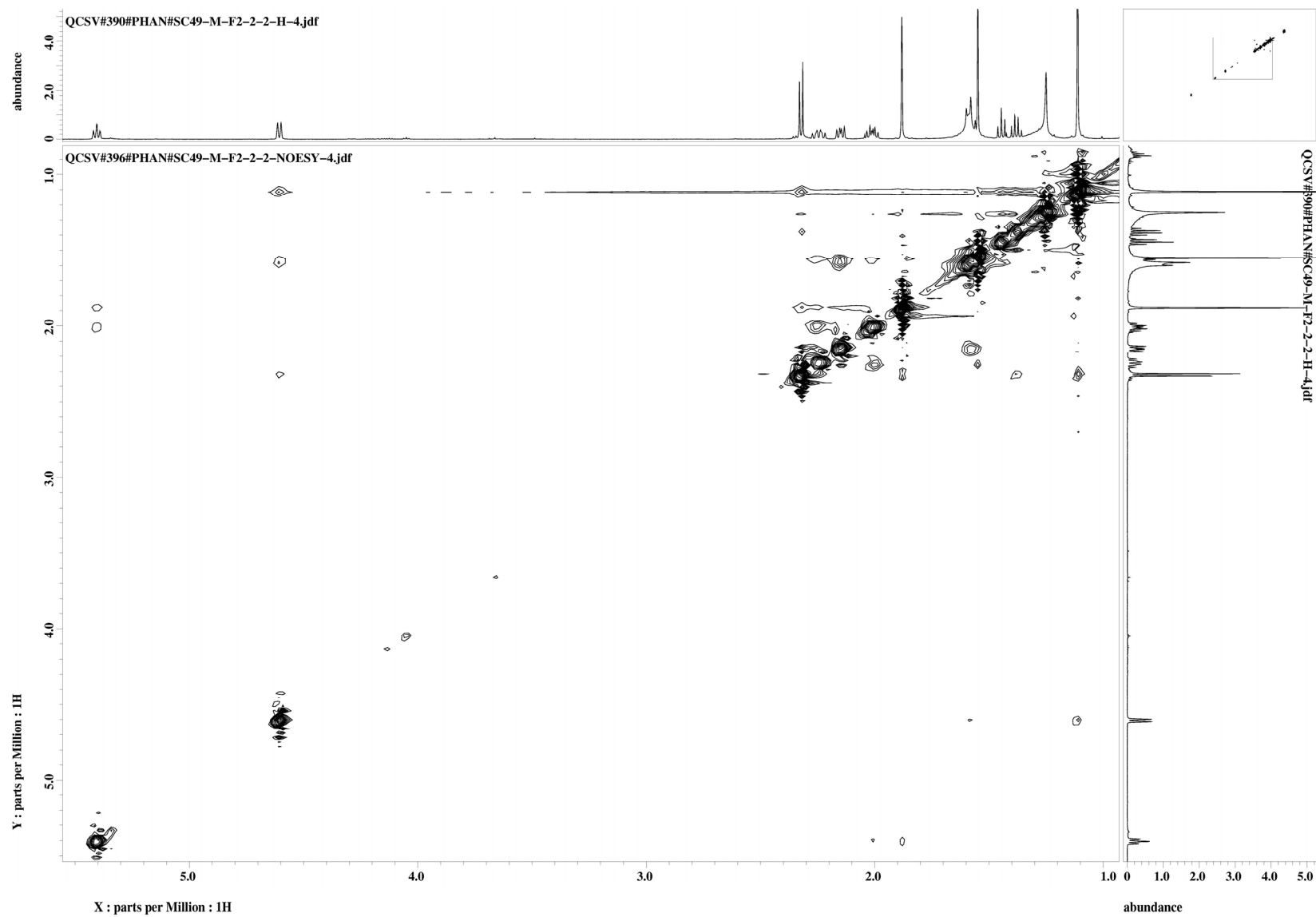
Figure S15. NOESY spectrum of capgermacrene B ( 2 ) in CDCl 3 .
