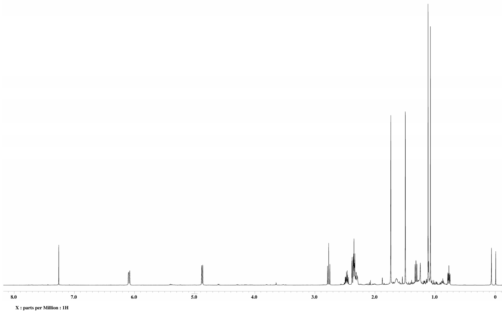
Figure S1. 1 H-NMR spectrum of capgermacrene A ( 1 ) in CDCl 3 (600 MHz).
