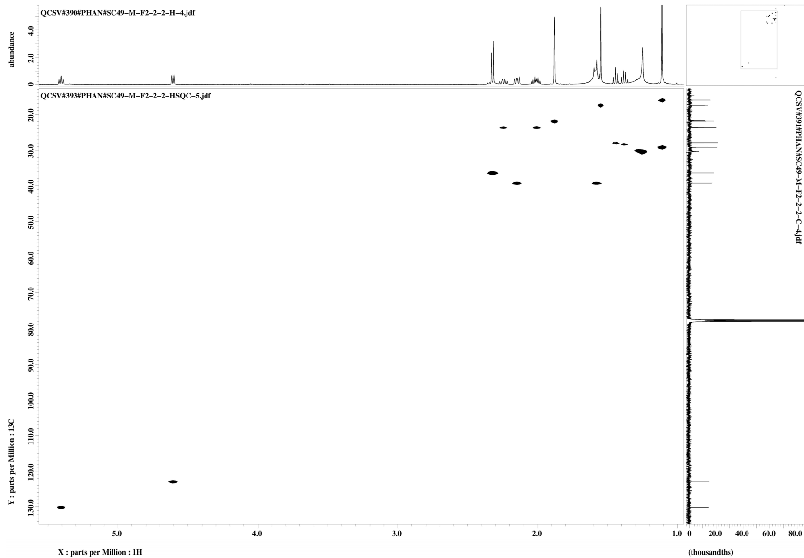
Figure S12. HSQC spectrum of capgermacrene B (2) in CDCl 3 .
