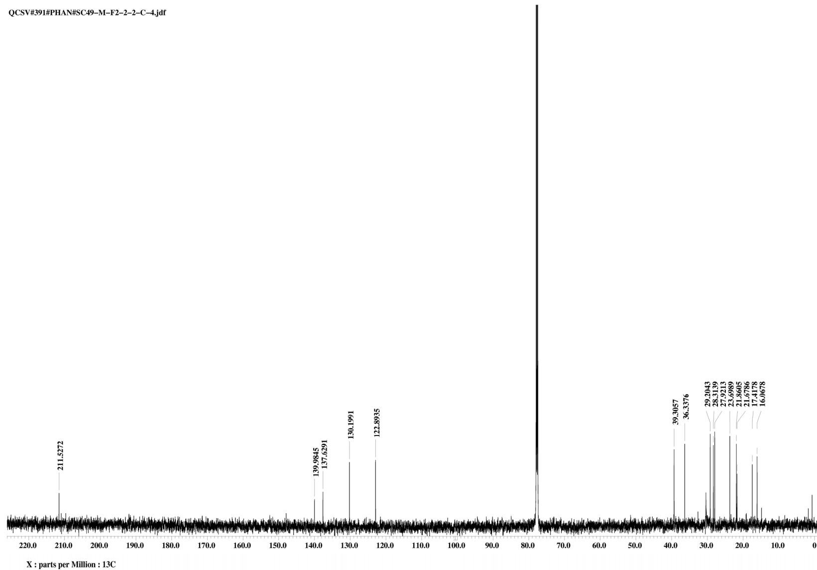
Figure S10. ^{13}\text{C} -NMR spectrum of capgermacrene B ( 2 ) in \text{CDCl}_3 (150 MHz).
