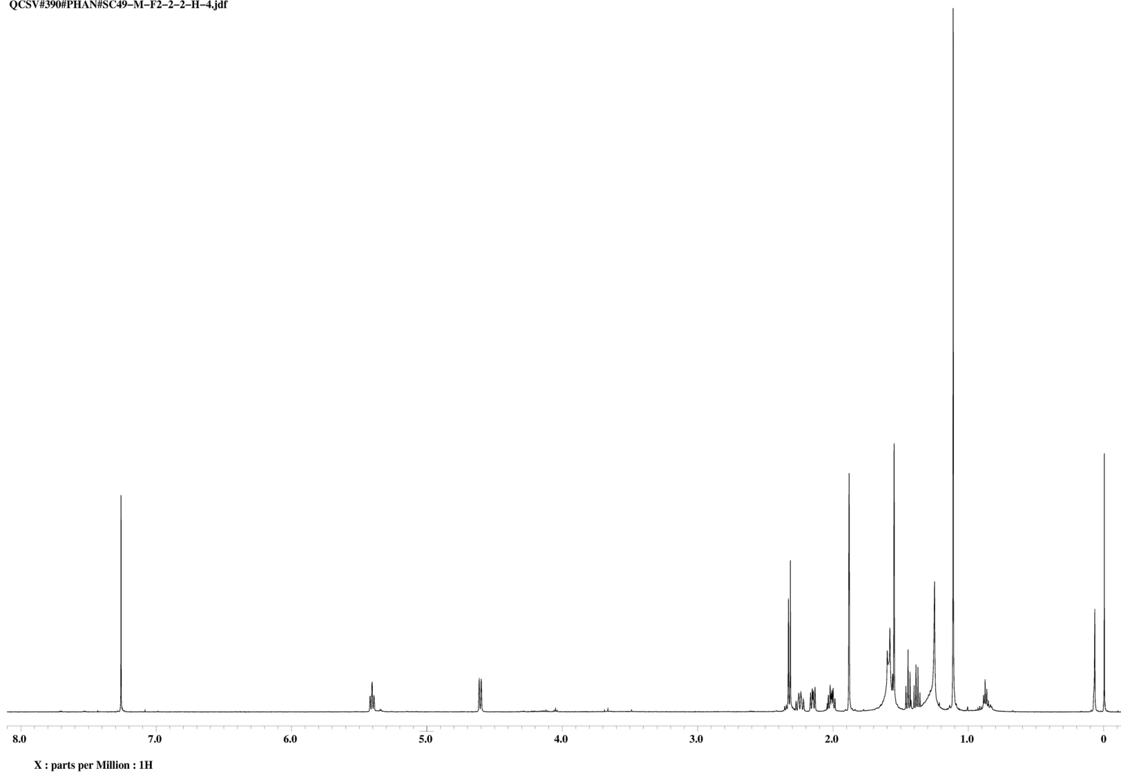
Figure S9. ^1\text{H} -NMR spectrum of capgermacrene B ( 2 ) in \text{CDCl}_3 (600 MHz).
