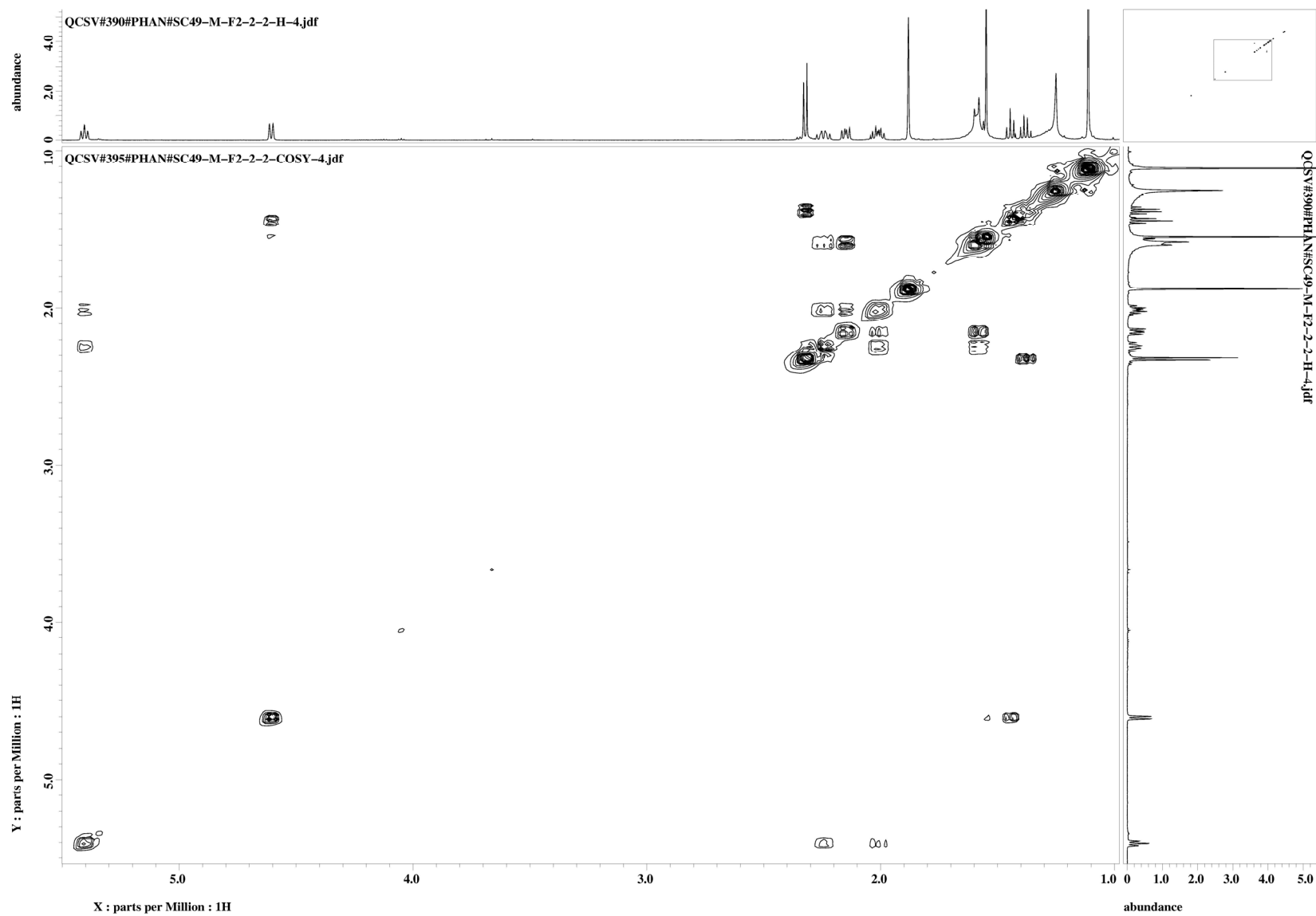
Figure S13. ^1\text{H} - ^1\text{H} COSY spectrum of capgermacrene B (2) in \text{CDCl}_3 .
