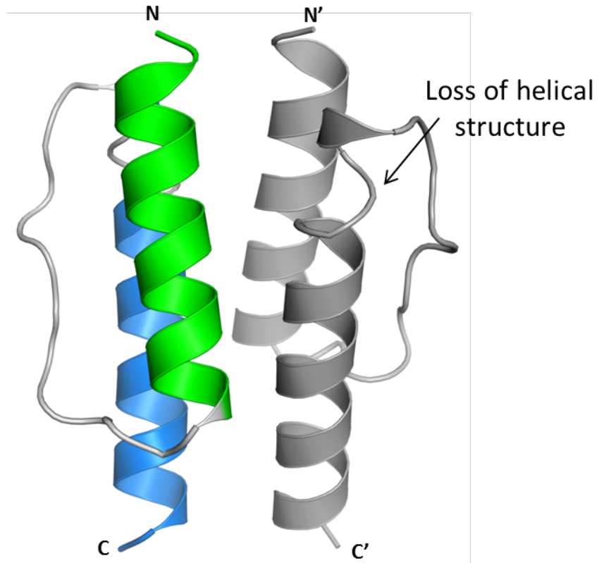
Figure S3. Model of PhoQ HAMP domain based on Aer2 HAMP1 L44H . One monomer is shown in color with \alpha 1 in green and \alpha 2 in blue, the other monomer is colored grey.
