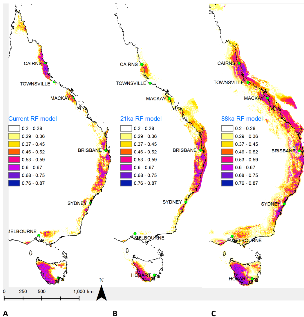
Figure S2. Distribution model for rainforest at 3 time periods. Note the large extent of rainforest in areas of current sea, which may have been important in maintaining continuity of rainforest habitat. (A) present model based on the pre-clearing extent of rainforest in Fig. S1(A). (B) projected to 21ka to represent a prediction for the last glacial maximum and (C) projected to 88ka to illustrate an earlier time of large estimated off-shore extent.
