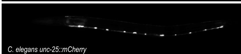
S2 Figure. Expression patterns directed by diverse unc-25 regulatory sequences in C. elegans . (A-C) C. elegans unc-25 regulatory sequence drives expression of mCherry in all transgenic strains; (A) M. hapla , (B) B. malayi , (C) T. spiralis unc-25 regulatory sequences drive expression of GFP . Animals photographed at 400x magnification. Images are mosaics of single animals.
