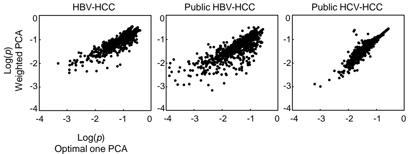
Figure S1. Comparison of one-optimal PCA and weighted PCA methods. Log-rank p -values of 882 pathways calculated with the two methods were compared. One-optimal PCA used one principal component optimally associated with recurrence while weighted PCA used multiple principal components explaining over 80% variance in each dataset.
