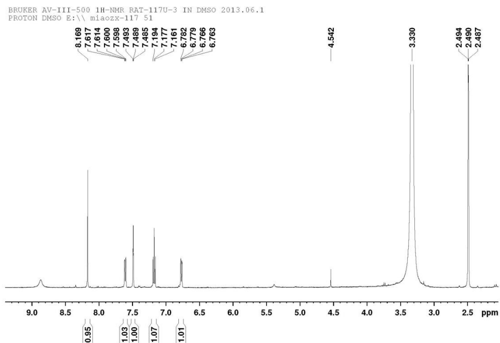
Fig. S3-2 ^1\text{H} NMR spectrum of M3 (500 MHz, DMSO, 25 ^\circ\text{C} ).
