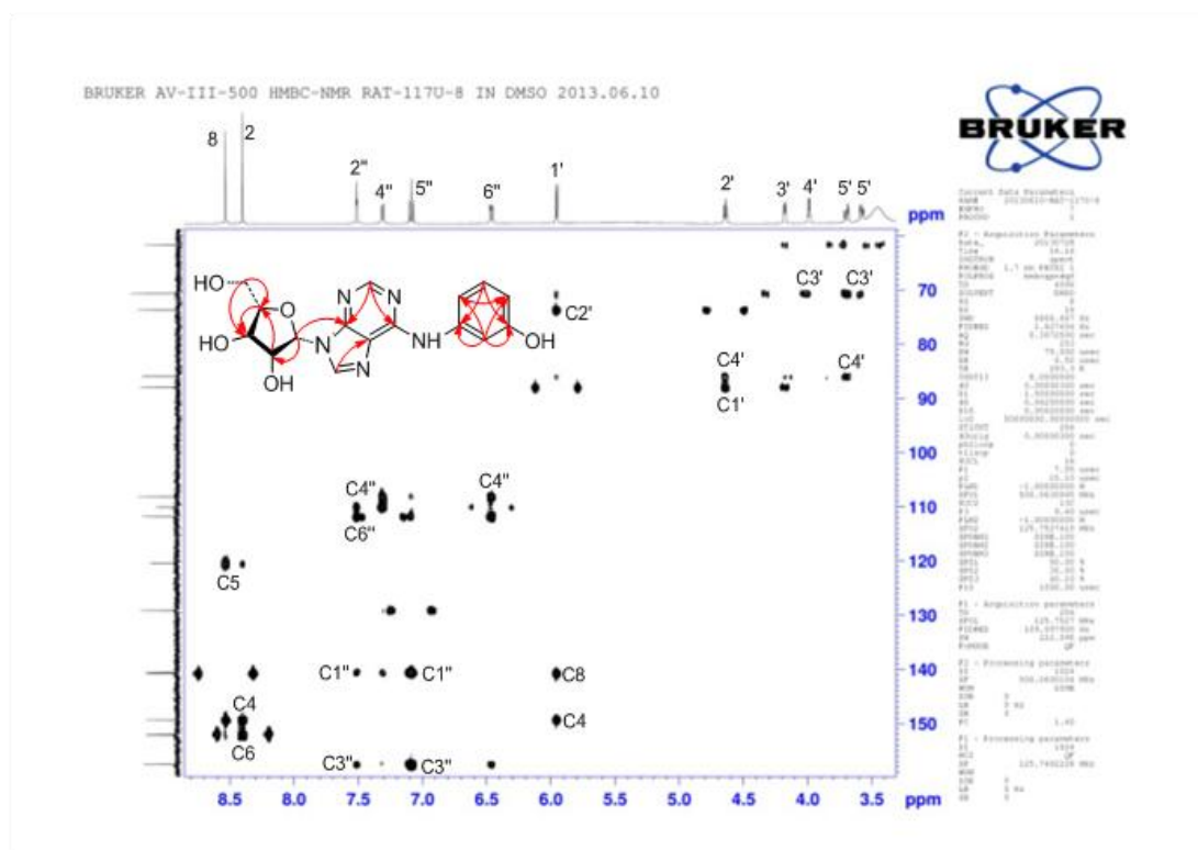
Fig. S8-8 HMBC NMR spectrum of M8 (500 MHz, DMSO, 25 °C).
