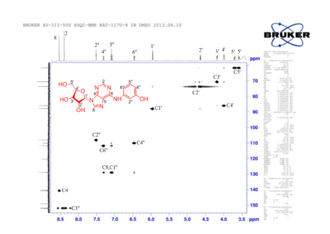
Fig. S8-7 HSQC NMR spectrum of M8 (500 MHz, DMSO, 25 °C).
