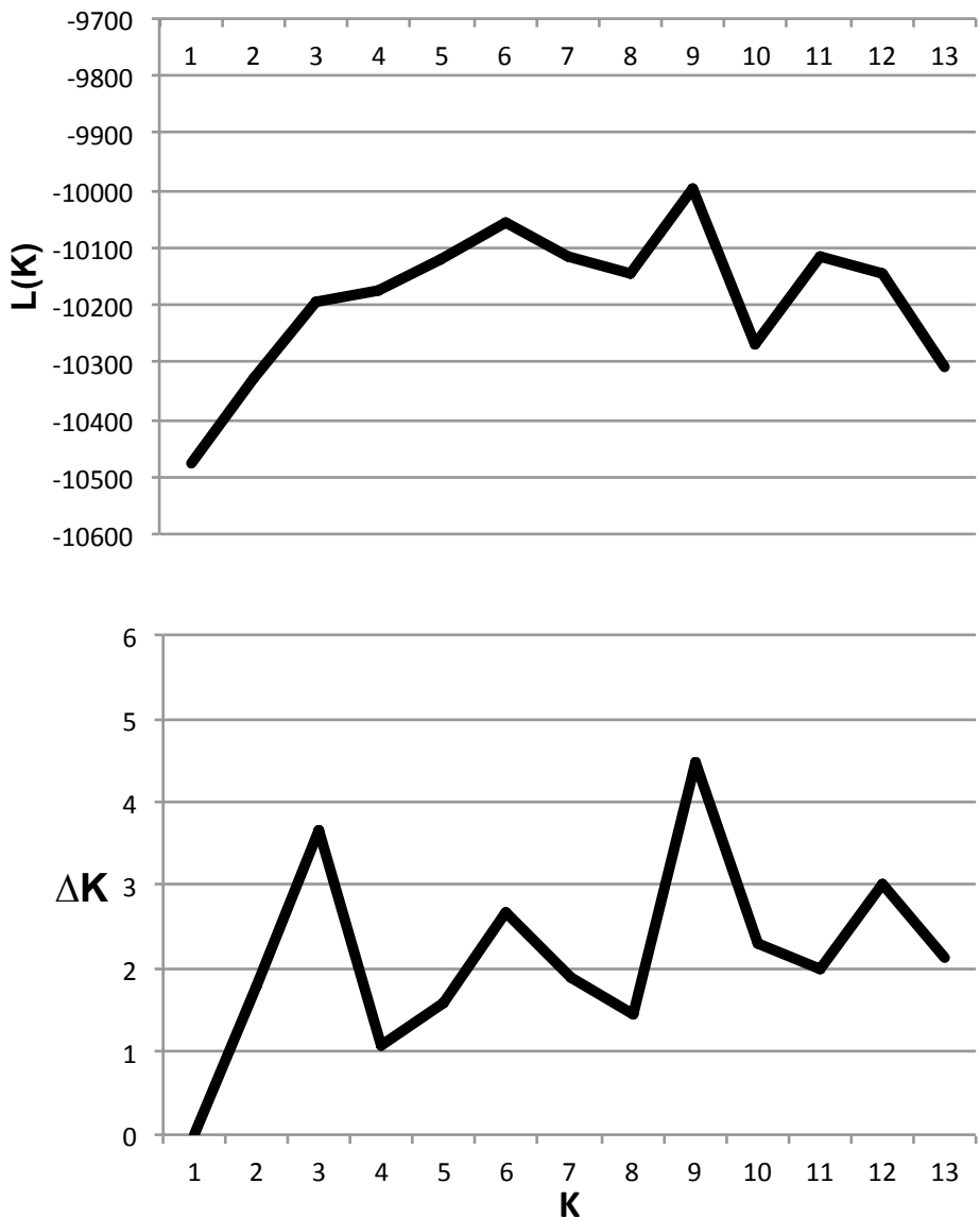
Fig. S1. L(K) and \Delta K at different values of K . Peaks of \Delta K were found at K=3, K=6, K=9 . B. L(K) are averaged over 10 independent replicates.
