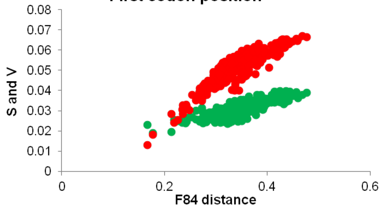
First codon position
