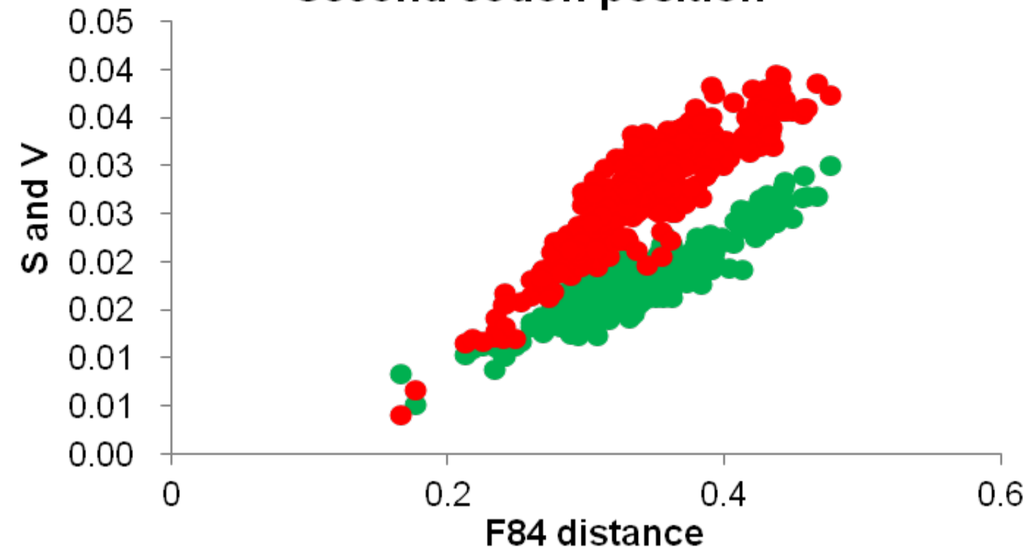
Second codon position
