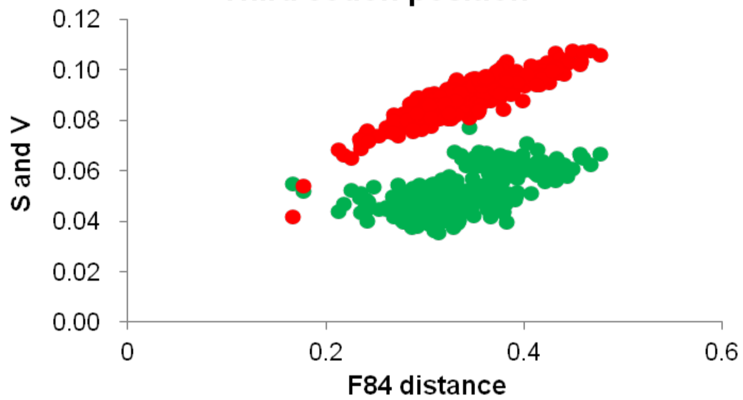
Third codon position
