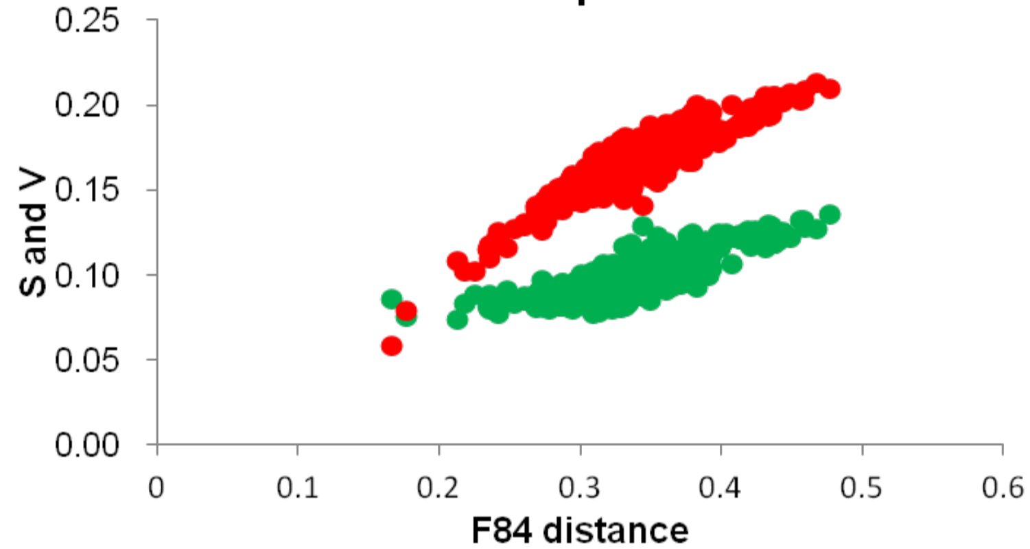
three codon positions
