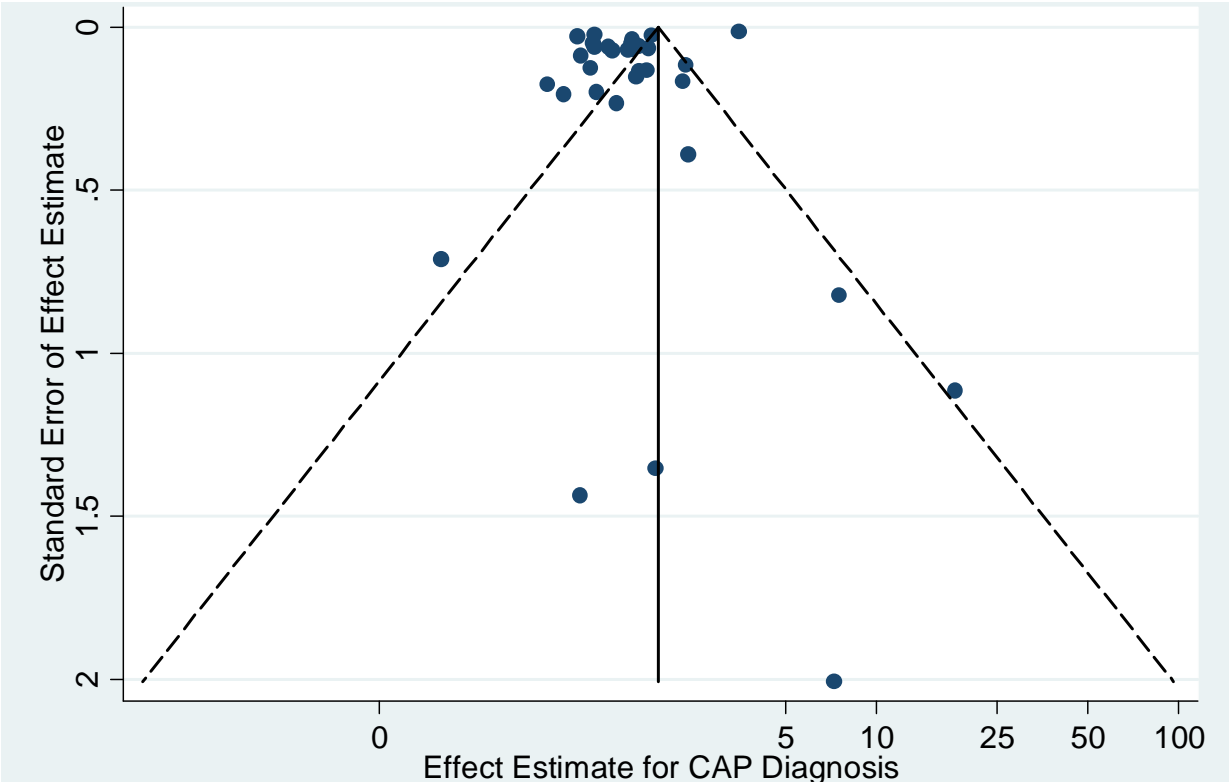
This funnel plot displays standard error of the effect estimate as a measure of study size on the vertical axis and estimated effect of PPI therapy on CAP diagnosis on the horizontal axis. Dashed lines represent pseudo-95% confidence interval lines, drawn around the summary fixed-effect estimate of the effect of PPI therapy on CAP diagnosis.
