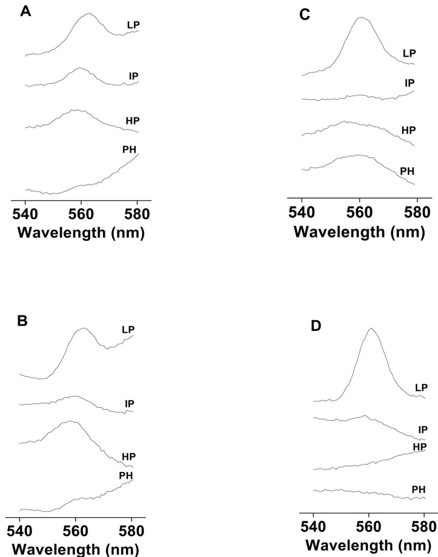
Fig. 4. The effects of DCMU and dinoseb on cyt b 559 photoreduction measured using unsupplemented and PQ-supplemented PSII membranes. Cyt b 559 photoreduction was measured using unsupplemented [A, C] and PQ-supplemented [B, D] PSII membranes in the presence of DCMU [A, B] and dinoseb [C, D]. The other experimental conditions were the same as described in Fig. 3.
