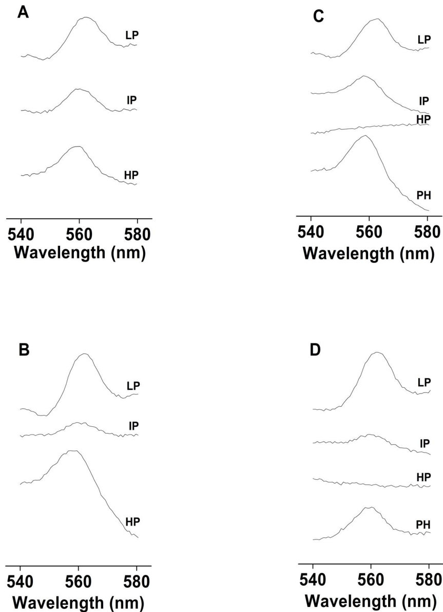
Fig. 3. Differences in redox spectra and cyt b 559 photoreduction measured using unsupplemented and PQ-supplemented PSII membranes. Differences in the redox spectra of cyt b 559 measured in the dark using unsupplemented [A] and PQ-supplemented PSII membranes [B]. 100 \mu M PQ-1 was added to the PSII membranes prior to the experiments. To measure cyt b 559 photoreduction, unsupplemented [C] and PQ-supplemented PSII membranes [D] were illuminated for 180 s at high light intensity (1000 \mu mol photons m^{-2} s^{-1} ). The spectra represent the difference in the light minus ferricyanide-oxidized spectra [the photoreduced HP form of cyt b 559 , (PH)], hydroquinone-reduced minus ferricyanide-oxidized or hydroquinone-reduced minus light spectra [HP form of cyt b 559 , (HP)], ascorbate-reduced minus hydroquinone-reduced spectra [IP form of cyt b 559 , (IP)] and dithionite-reduced minus ascorbate-reduced spectra [LP form of cyt b 559 , (LP)].
