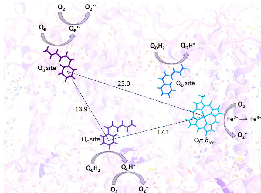
Fig. 5. Proposed mechanism for the involvement of loosely bound plastosemiquinone at the Q_B and Q_C sites in O_2^{\cdot -} formation in PSII. Superoxide anion radicals are produced via one-electron reduction of molecular oxygen by plastosemiquinones, which are formed via one-electron reduction of plastoquinone at the Q_B sites and one-electron oxidation of plastoquinol at the Q_C site but unlikely at the Q_D site.
