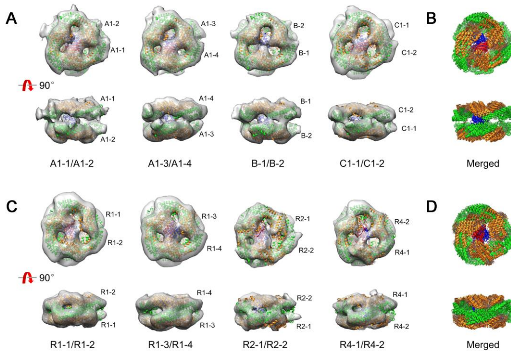
Fig. S6. Comparison of hexamers.
