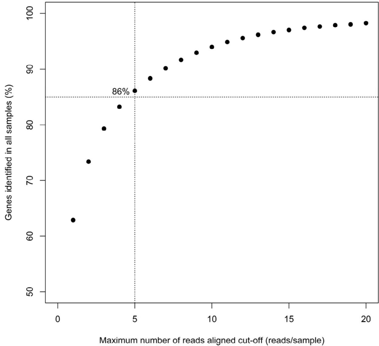
Supplementary Figure 1 Influence of minimum RNA-Seq aligned read threshold on the inclusion of genes detected in all samples. At a minimum of 5 aligned reads to call a gene “expressed or detected”, 86% of genes included in the analysis were detected in all samples.
