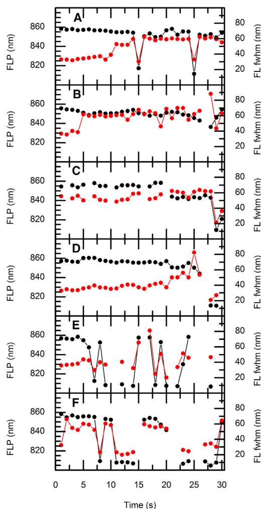
FIGURE 3 Temporal traces of the maximum FLP position ( black traces ) and width (FWHM, red traces ) of six LH2 proteins (A–F) equilibrated in the pH 7.5 buffer. The Gaps in the traces are due to fluorescence intermittency (i.e., quenched states when no fluorescence emission is observed). T = 287 K.
