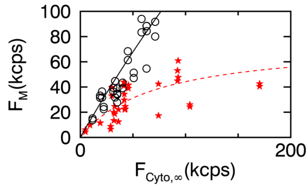
Figure S1: Close-up view of the low cytoplasmic intensity region of Figure 5A. Binding curve for EGFP-PCL \delta -PH (open circles) and fit (solid line) are shown together with the competitive binding curve for EGFP-PCL \delta -PH coexpressed with MiniGAP-mCh (solid stars) and fit (dotted line).
