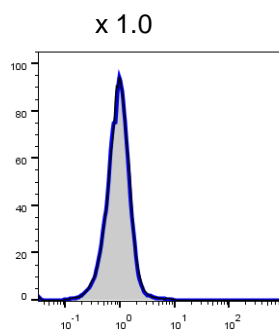
Parental K562
