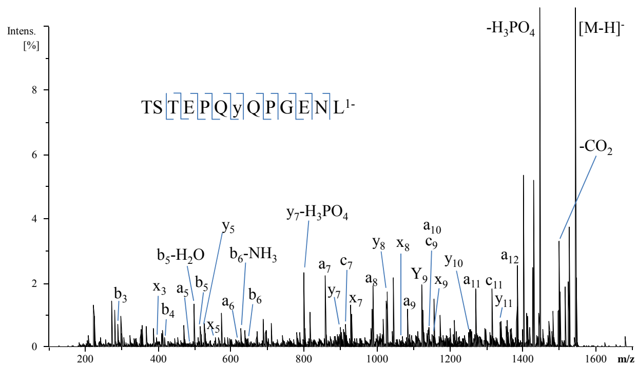
Supplemental Figure 1. UVPD spectrum of singly deprotonated TSTEPQyQPGENL.
