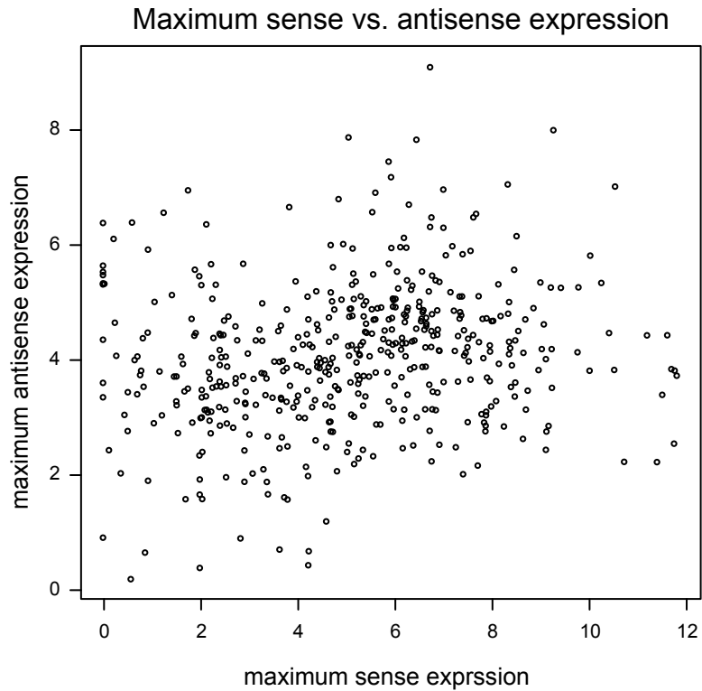
Figure S38. Maximum antisense expression level does not strongly correlate with maximum sense expression level. Each point represents a bidirectionally transcribed (sense and antisense) gene. We compared maximum sense and antisense transcript levels during the 56-hour time course. Expression is plotted in units of \log_2(\text{FPKM}+1) .
