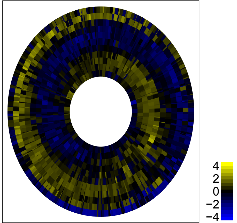
Figure S39. Periodicity is evident in P. falciparum blood stage expression profiles. For differentially expressed annotated mRNA genes, we visualized mean-centered expression profiles across the 56-hour time course in a circular, non-clustering heatmap. Genes are ordered by their angular position in the MDS plot of gene expression profiles and samples are ordered by time. Expression is in units of \log_2(\text{FPKM}+1) .
