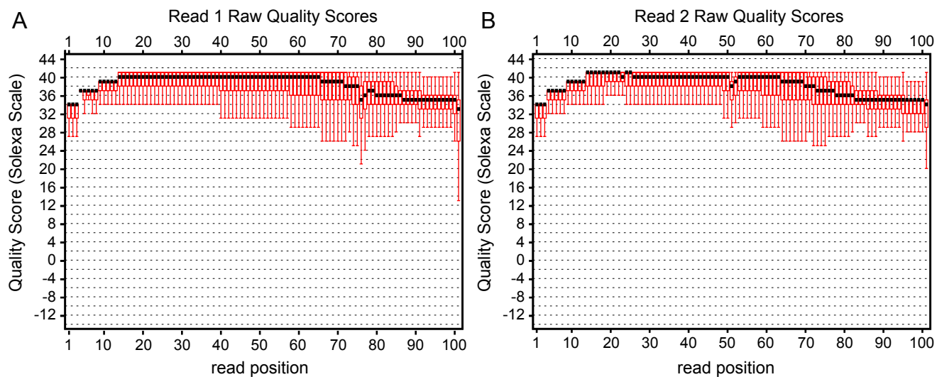
Figure S5. Raw reads have high quality scores. (A/B) Read 1 and Read 2 raw quality scores, respectively. Each plot summarizes approximately 307 million reads agglomerated from all fifteen samples. We trimmed the last base and filtered the 4-8% of reads from each sample that did not pass Illumina filtering prior to read alignment.
