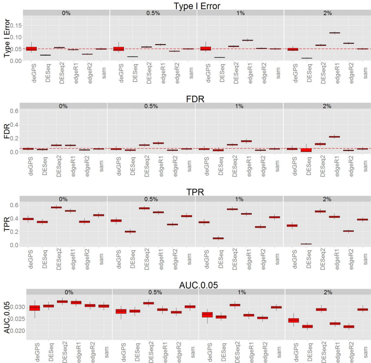
Figure S5. Simulation results from compcodeR. Sample size was set as 8 subjects per group. Note that edgeR2 does not control correct type I error when increasing sample size although its FDR is at the desired level.
