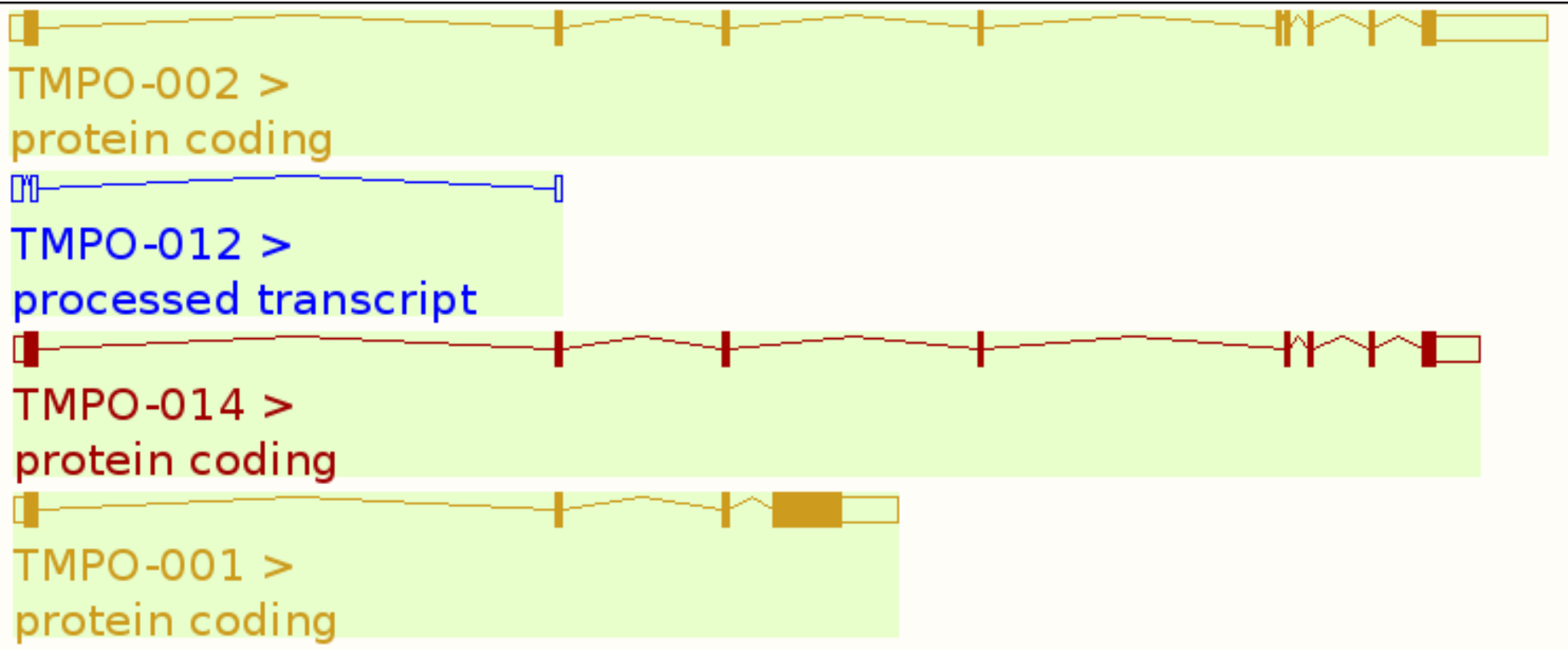
Figure S4. C-terminal substitution for TMPO .
