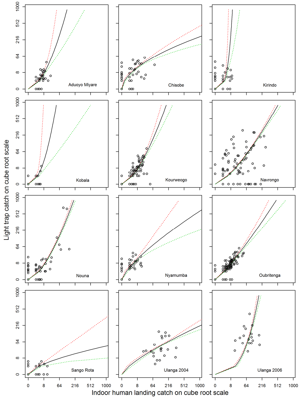
Figure A1. Site specific plots of the number of An. gambiae s.l. sampled by LT against those sampled by HLC, the straight line describes the relationship based on model 2.
