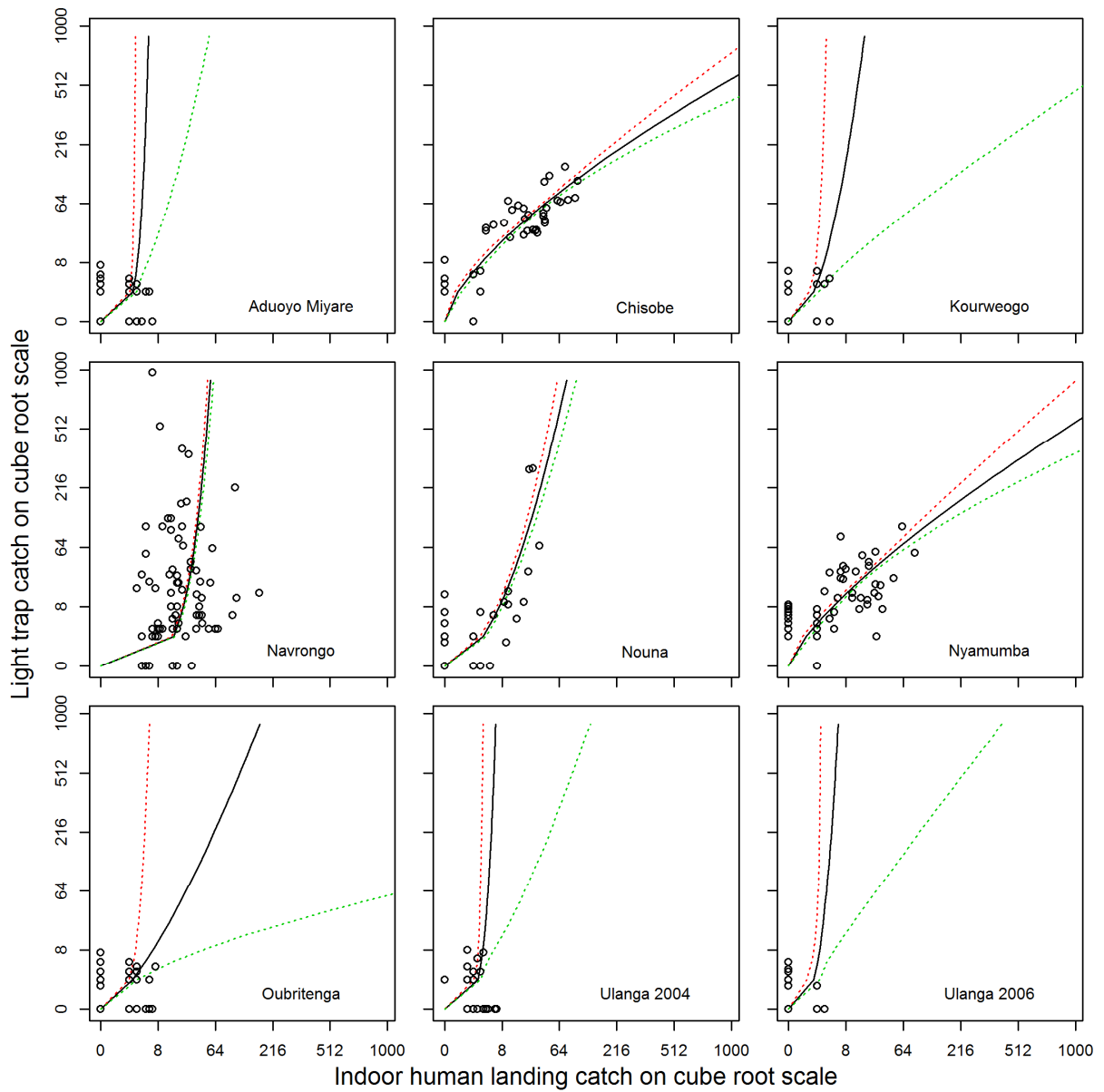
Figure A2. Site specific plots of the number of An. funestus s.l. sampled by LT against those sampled by HLC, the straight line describes the relationship based on model 2.
