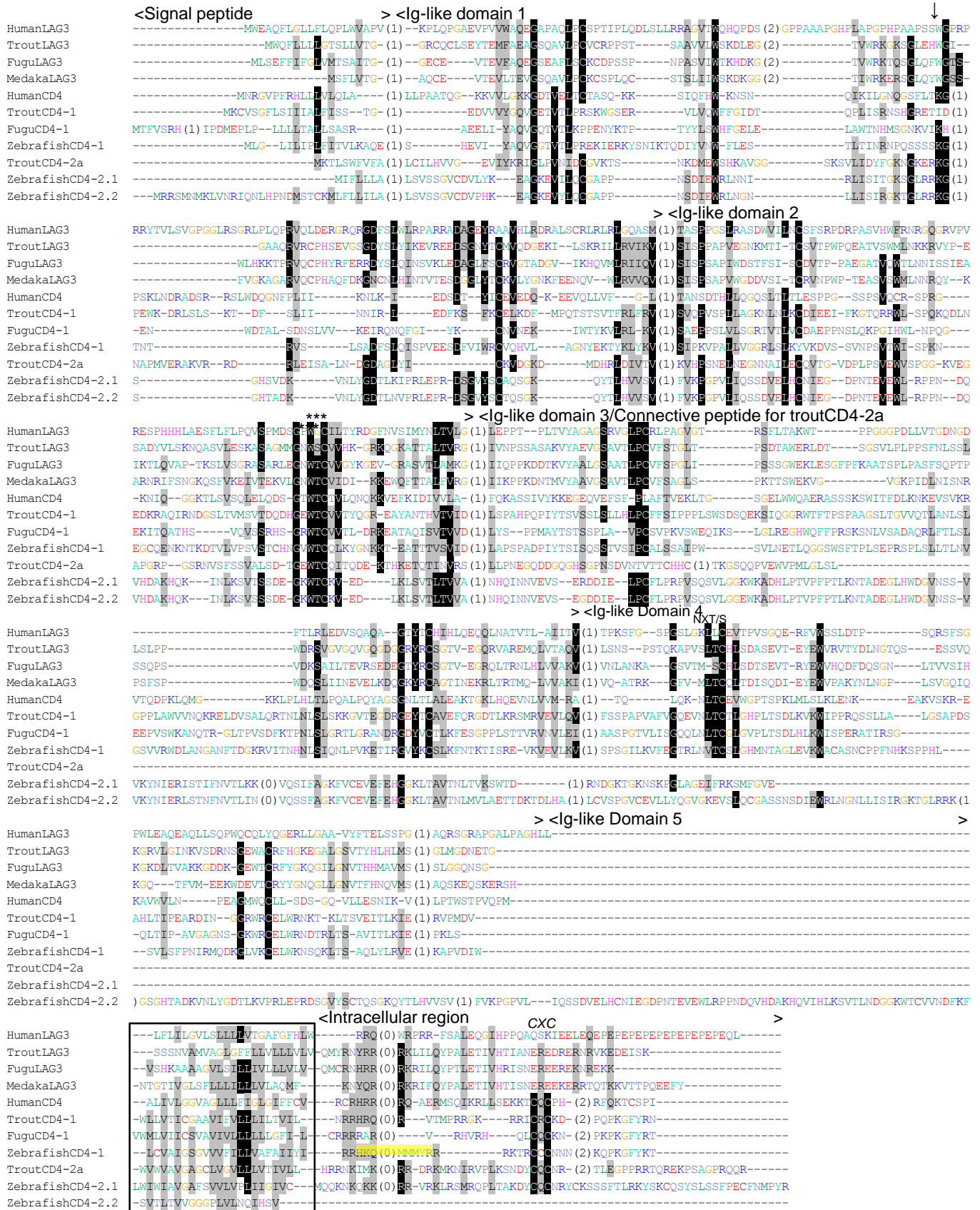
Figure S4. Multiple sequence alignment of zfCD4 proteins with other CD4 and LAG3 homologues. The Ick binding site (CXC) is labelled above the sequence in italics and Lys46 for CD4 is indicated with an arrow above the sequence. Other conserved regions include the WTC, marked with asterisks, and N-linked glycosylation sites (NXT/S), labelled above the sequence. The transmembrane domain is boxed and identified as amphipathic alpha-helix motif is highlighted in yellow. (x) indicate intron position with intron phase.
