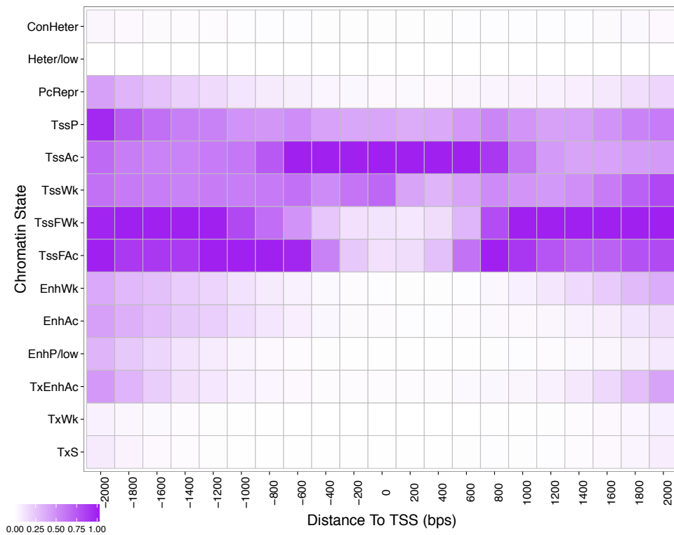
S3 Fig. Supporting matrices for the 14 chromatin states map of brain. (A) The transition probability matrix indicating the probabilities of each 200-bp (bin size) region switching from one state to another. (B) The probability matrix representing the probabilities of each 200-bp (bin size) region to be within 2kb (upstream and downstream) of the transcription start sites.
