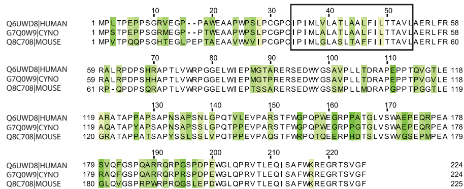
Figure S1. Multiple sequence alignment of SAIL protein between human, cynomolgus monkey and mouse. The Uniprot Accession Numbers for the input sequences are shown. Green-shaded boxes indicate divergent sequences. Predicted transmembrane domain is highlighted by black box.
