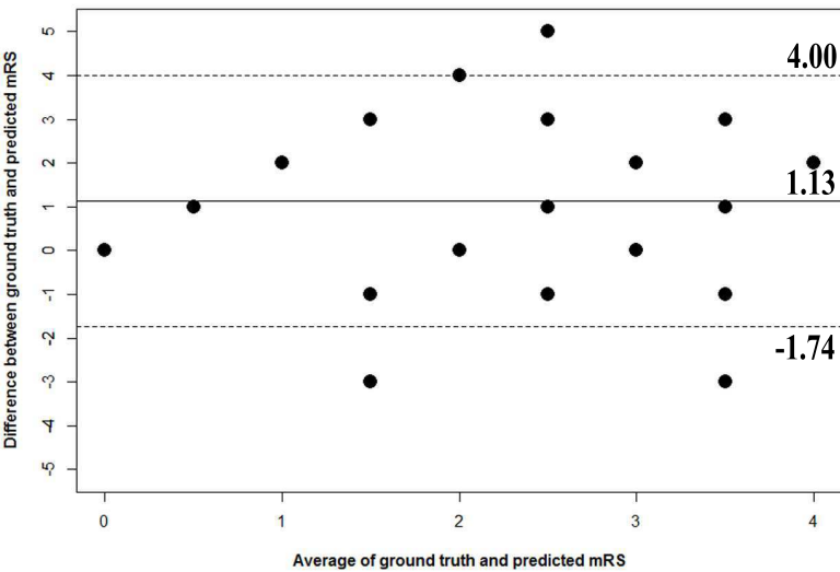
VLSM Model
