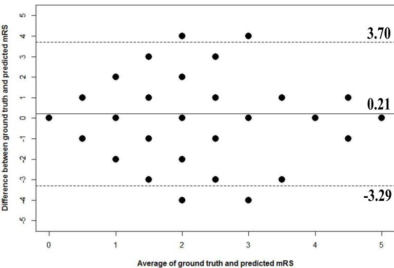
Problem-specific Model
