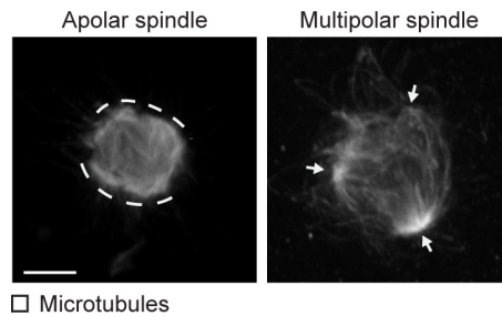
Fig. S6. Apolar and multipolar spindles in fixed human oocytes.
