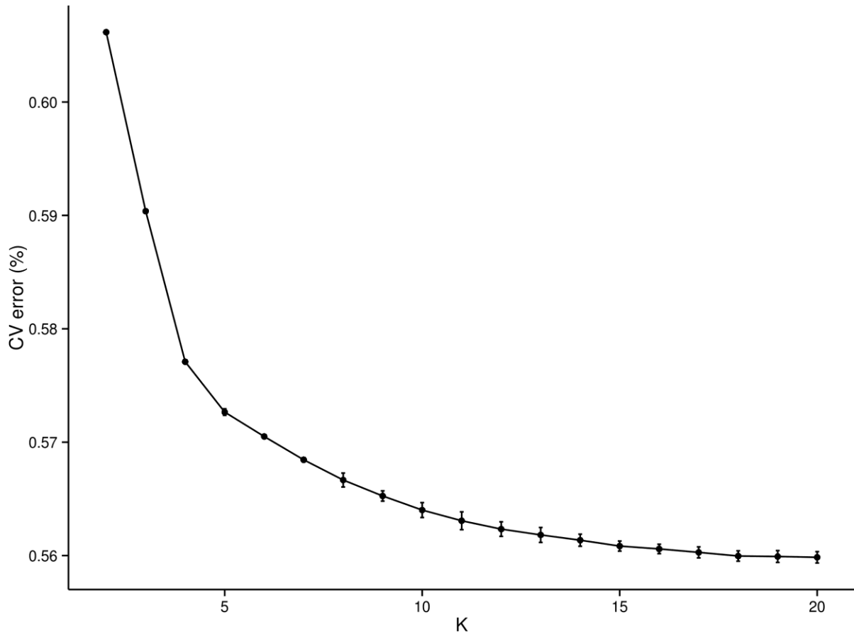
Supplementary Figure 1: Selection of the optimal number of admixture components, ten-fold cross-validation (CV), K=2..20.
