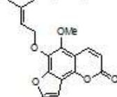
6-isopentenylxyisobergaptol
