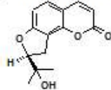
Isobergaptol
