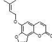
Heratomine
