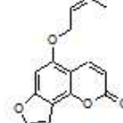
Lanatine
