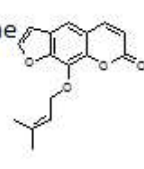
8-methylpsoralen
