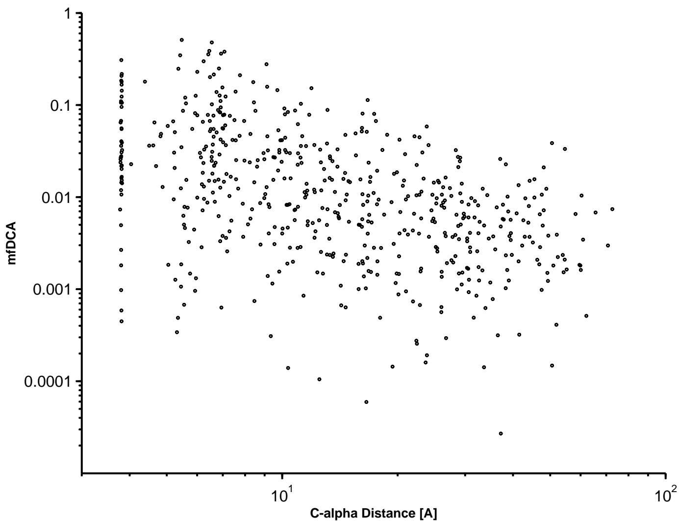
S8 Fig. As expected, the intensity of the mfDCA correlation for the significant couplings decreased with the distance and this decrease was roughly proportional to the square of the distance between the Ca atoms of the residues.
