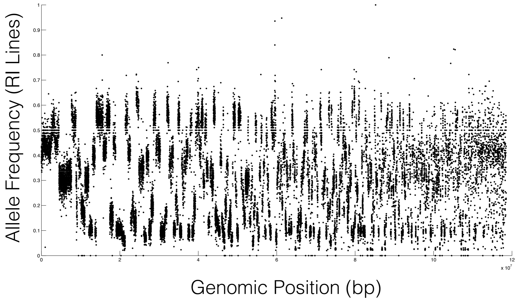
S5 Figure. Allele frequencies for every RAD-associated SNP marker.} Markers are plotted along each scaffold and scaffolds are ordered by length.
