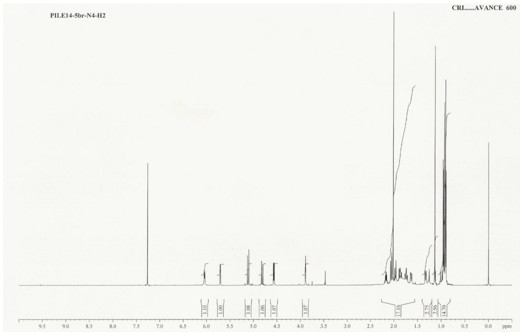
Figure S3. 1 H NMR spectrum (CDCl 3 ) of compound 4.
