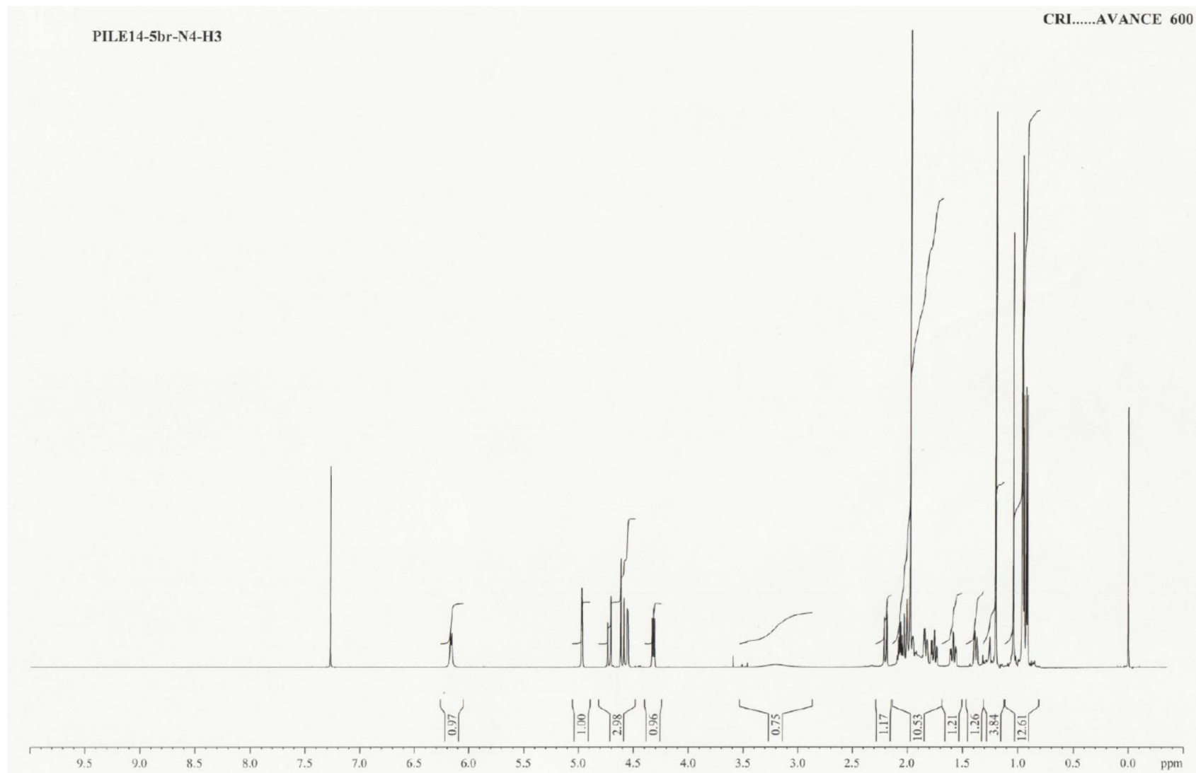
Figure S9. 1 H NMR spectrum (CDCl 3 ) of compound 7.
