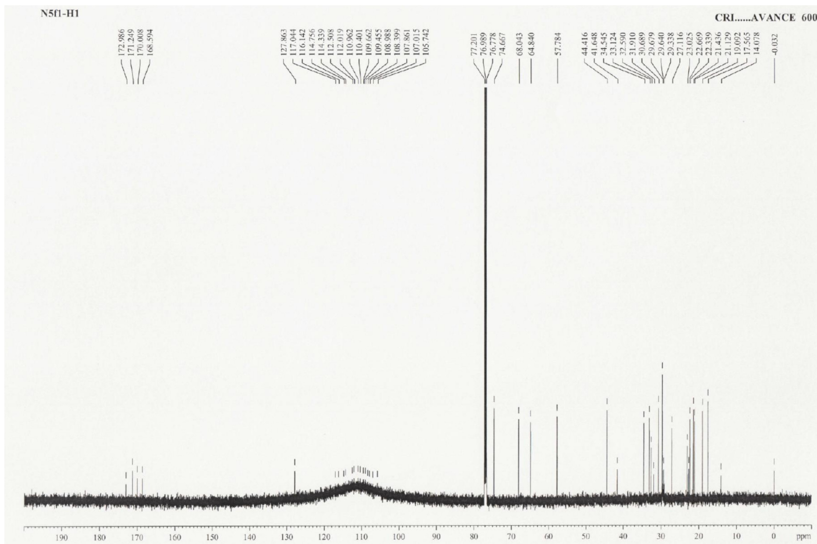
Figure S8. ^{13}\text{C} NMR spectrum ( \text{CDCl}_3 ) of compound 6 .
