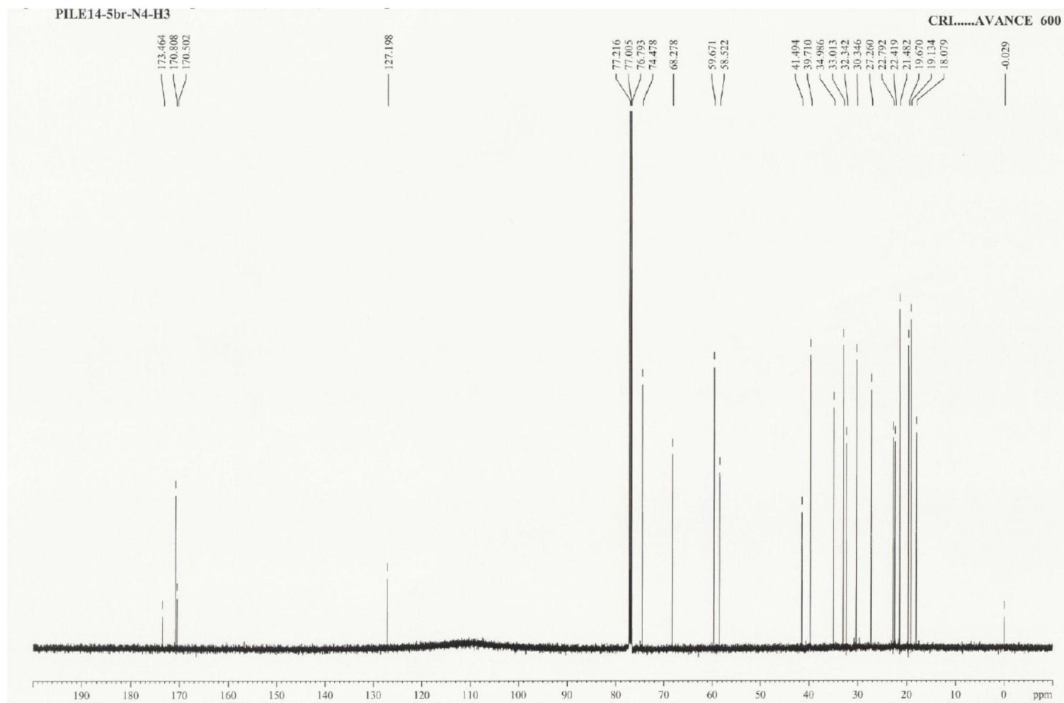
Figure S10. ^{13}\text{C} NMR spectrum ( \text{CDCl}_3 ) of compound 7.
