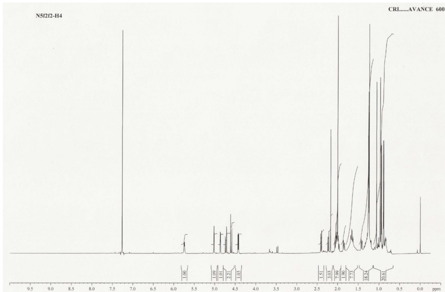
Figure S1. ^1\text{H} NMR spectrum ( \text{CDCl}_3 ) of compound 3.
