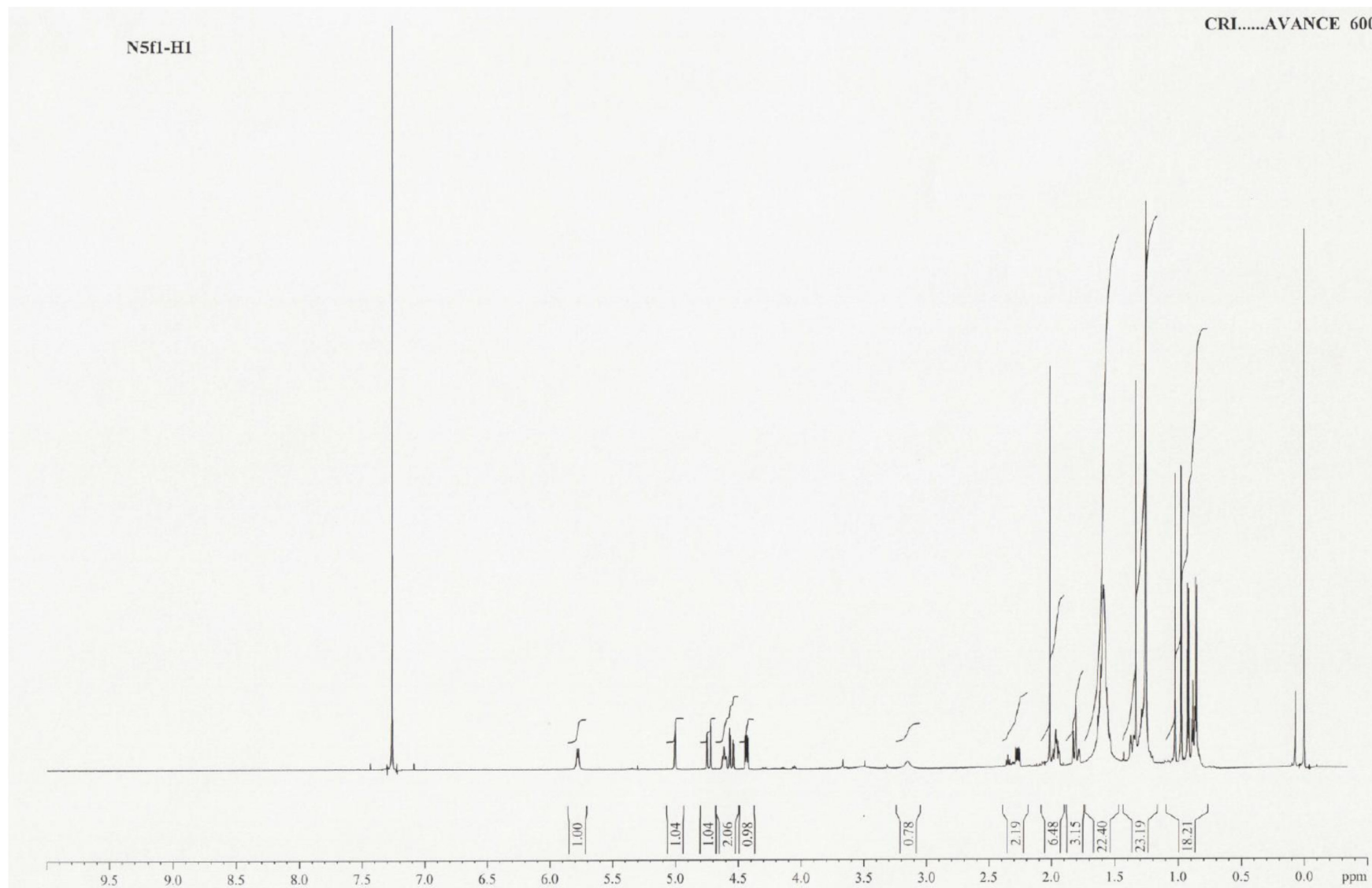
Figure S7. 1 H NMR spectrum (CDCl 3 ) of compound 6.
