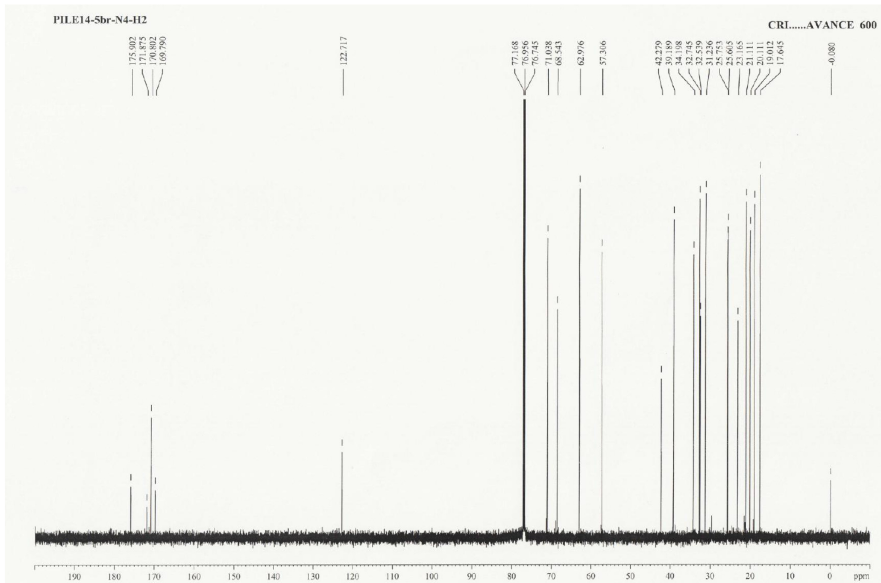
Figure S4. ^{13}\text{C} NMR spectrum ( \text{CDCl}_3 ) of compound 4.
