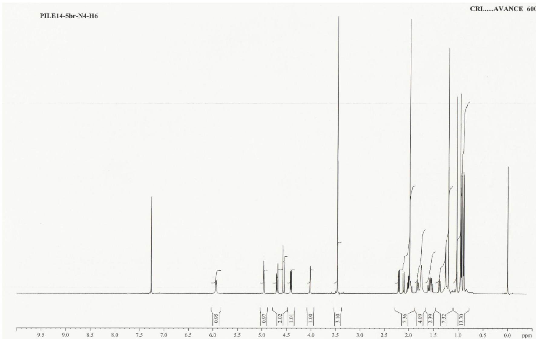
Figure S5. 1 H NMR spectrum (CDCl 3 ) of compound 5.
