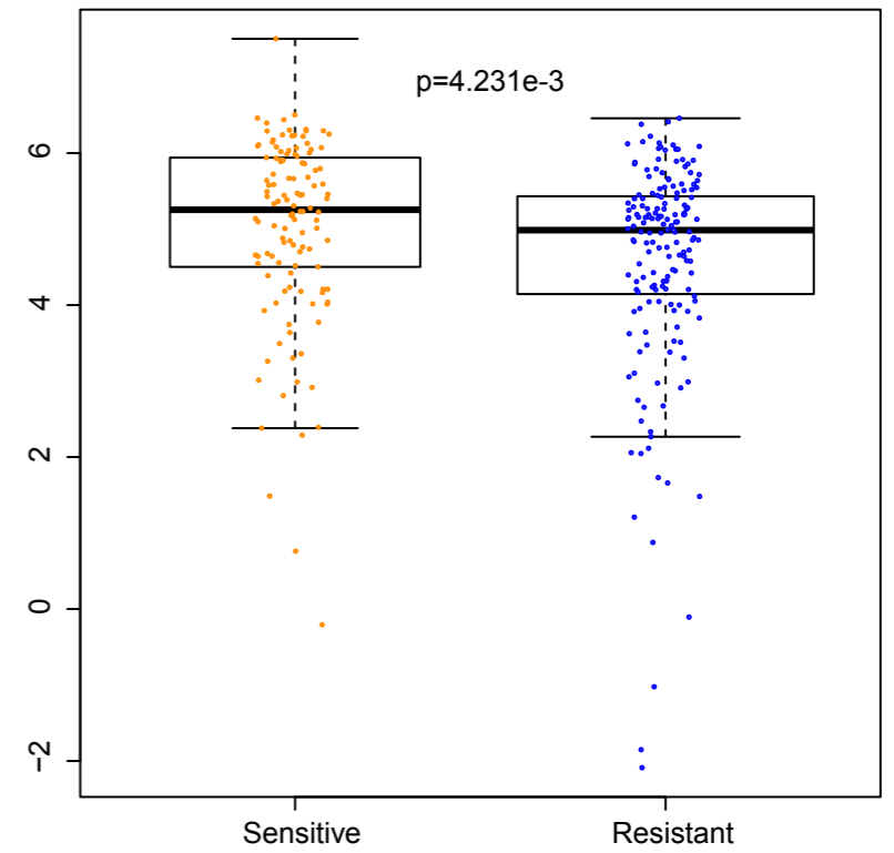
PHA-665752
