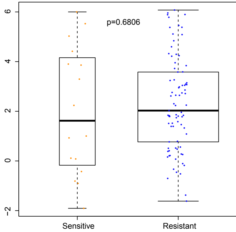
PD-0332991
