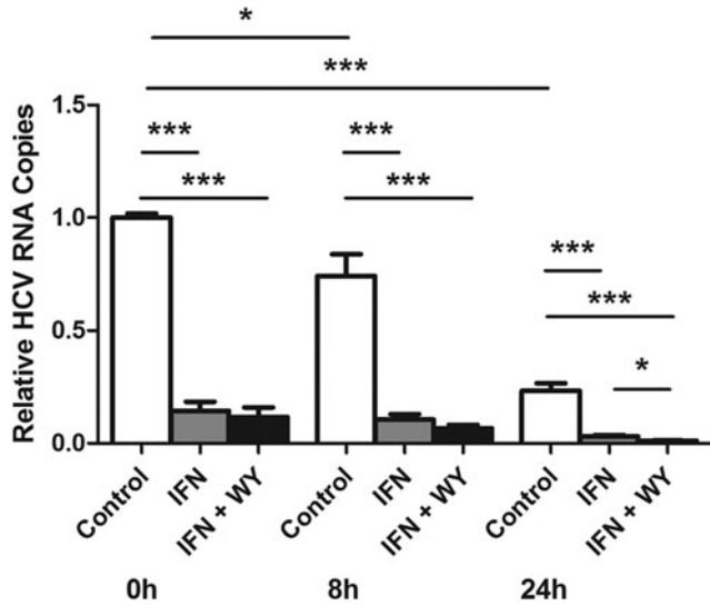
SUPPLEMENTARY FIG. S1. IFN pretreatment in combination with WY-14643 reduces HCV replication. JFH1-infected Huh-7 cells were mock treated or treated with 2 U/mL IFN- \alpha \pm WY-14643 for 3 weeks, followed by 20 U/mL IFN- \alpha . IFN- \alpha pretreatment significantly reduced JFH1 replication at all time points compared with the mock-treated control. The addition of WY-14643 to IFN- \alpha pretreatment significantly reduced HCV RNA copies 24 h posttreatment with 20 U/mL IFN- \alpha (* P < 0.05; ** P < 0.01).
