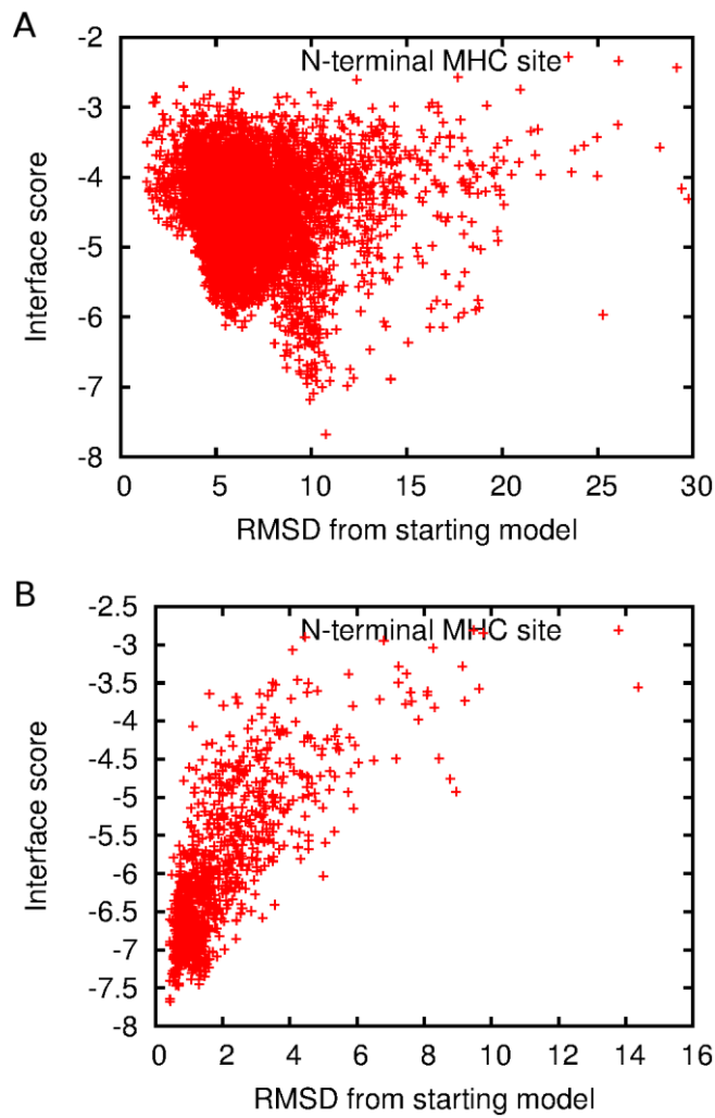
S1 Fig. MHC modeled at the N-terminal site of SEE-TCR. (A) Initial generation of 5000 models, plotted after interface score versus RMSD from the starting model. (B) Generation of 1000 models with the final model as starting point, to verify presence of a local energy minimum.
