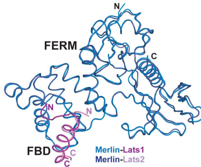
Supplementary information, Figure S4. Comparison of the structures of the Merlin-FERM/Lats1 and Merlin-FERM/Lats2 complexes.
