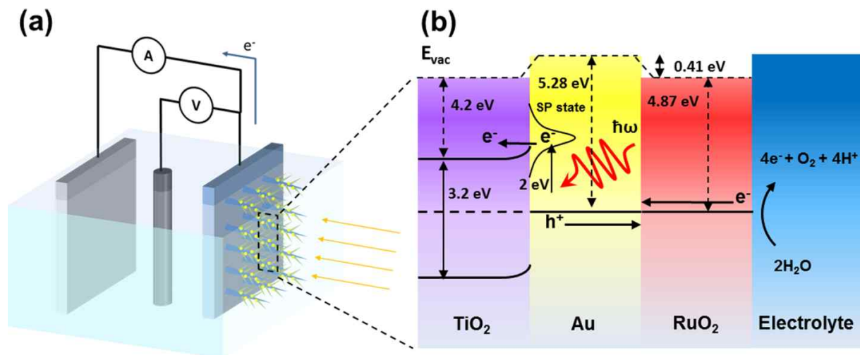
Figure S2. (a) Schematic diagram of electrochemical cell for voltammetry. (b) Schematic energy level diagram of plasmonic system with OEC for solar water splitting.
