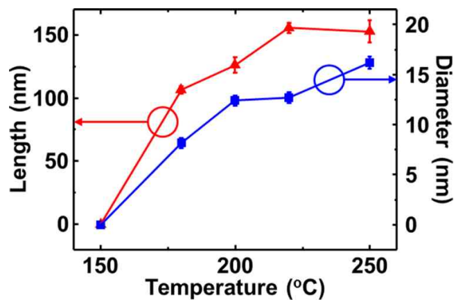
Figure S1. The length and diameter of RuO 2 nanowires with the annealing temperature.
