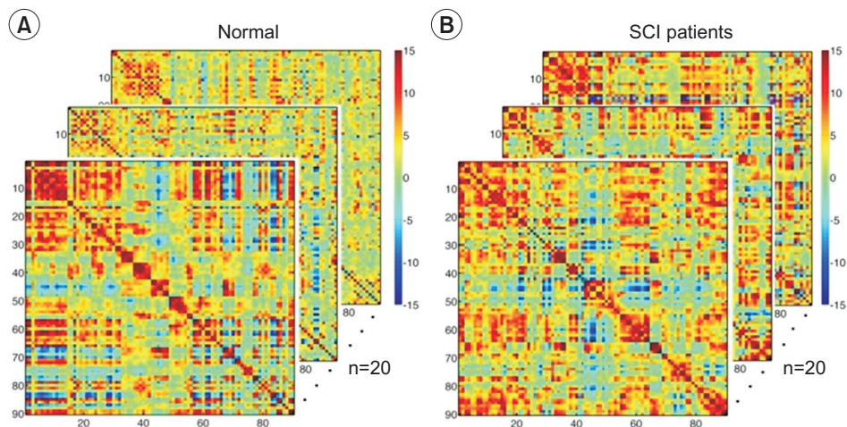
Supplementary Fig. 1. Correlation matrix in both of the control (A) and spinal cord injury (SCI) patients (B). The x-axis and y-axis means specific region of interests according to an automated anatomical labeling template. The sequential order of each axis is represented in Supplementary Table 1. The color bar means z-score. The positive functional connectivity between two regions is represented in red and the negative functional connectivity is represented in blue.
